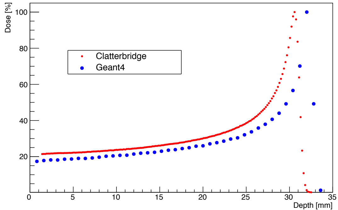
Bragg peak
