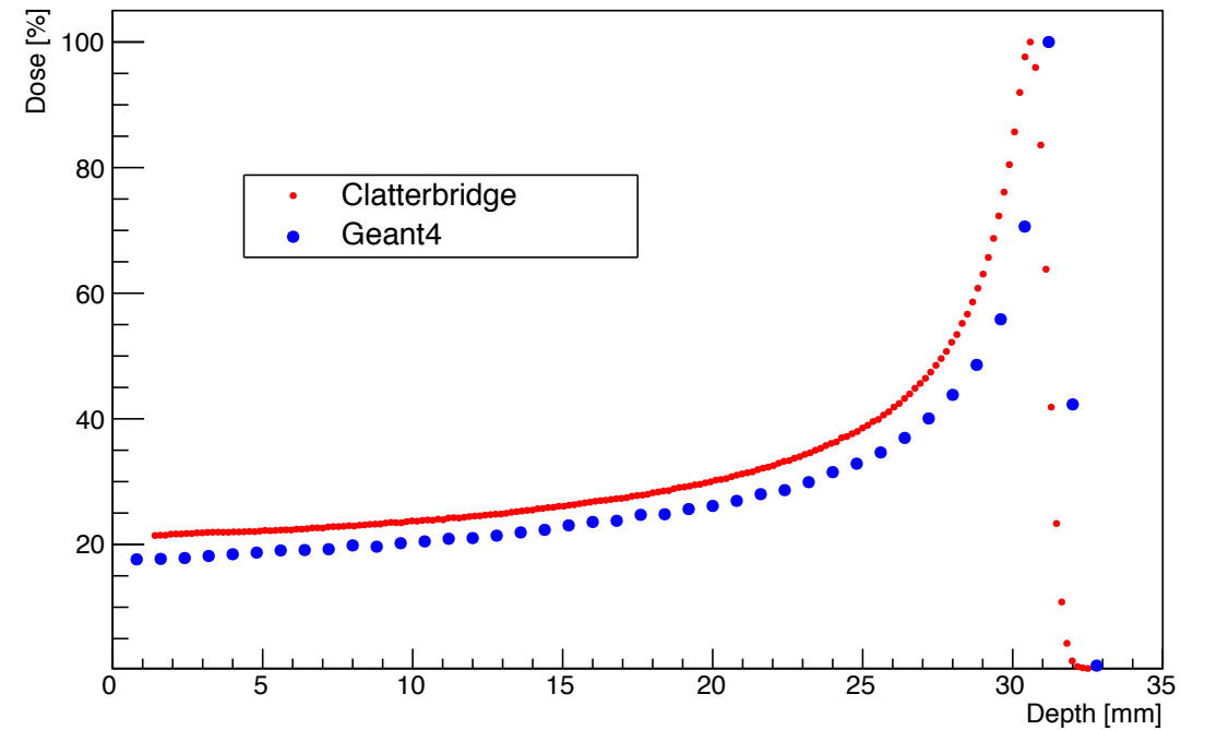
Bragg peak
