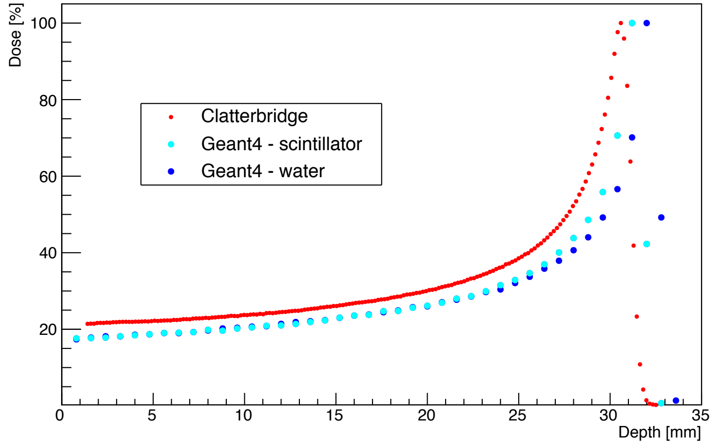
Bragg peak
