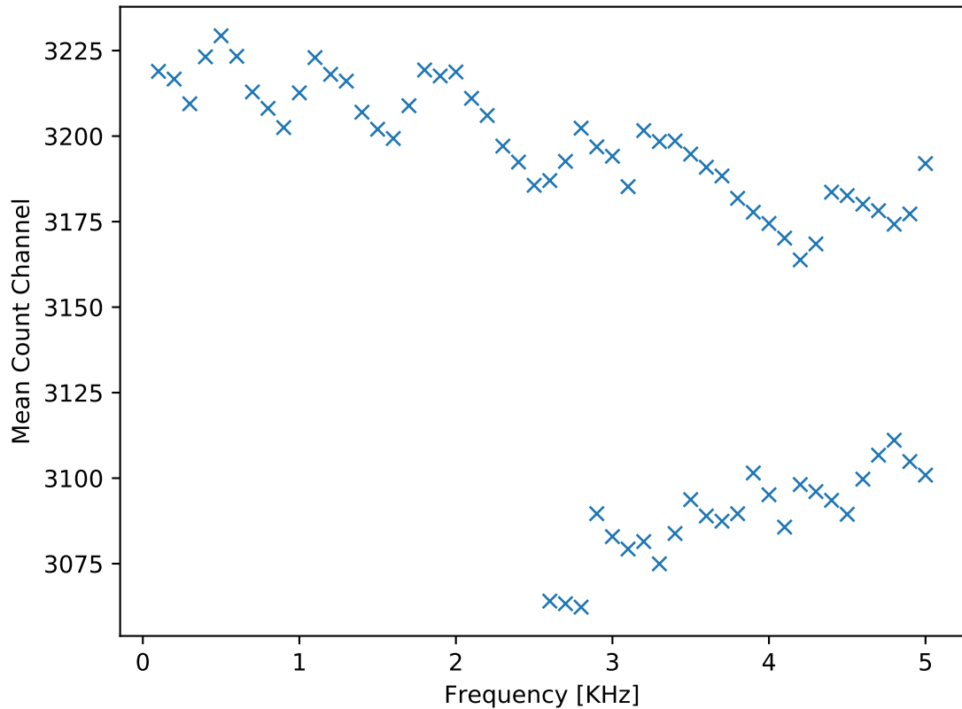
Hamamatsu PMT - Self Trigger - 2.14V - 900V
