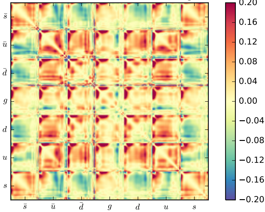
Correlations META30-META900 NNLO @ 8 GeV
