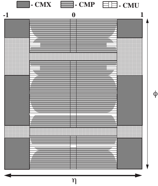
Figure 2.5: The coverage of the muon chambers in the \eta - \phi plane.
