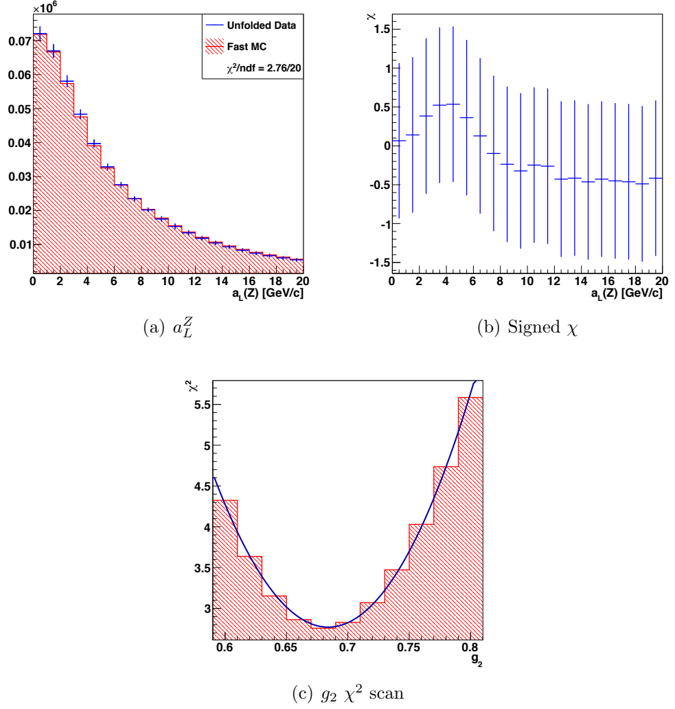
Figure 8.13: The best \chi^2 fit between the background subtracted and unfolded Z^0 \rightarrow e^+e^- data and g_2 -reweighted fast Monte Carlo using the KN global fit parameters for g_1 and g_3 . One iteration of the unfolding algorithm has been used to unfold the data.
