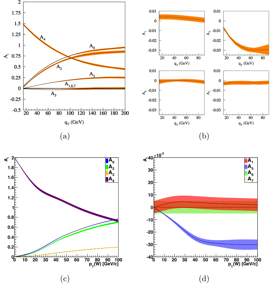
Figure 6.2: The evolution of the A_i coefficient in p_T^W . (a) and (b) show the functions obtained in [77], (c) and (d) show the implementation of these coefficients in the fast simulation. In both cases the shaded regions indicate the uncertainty.
