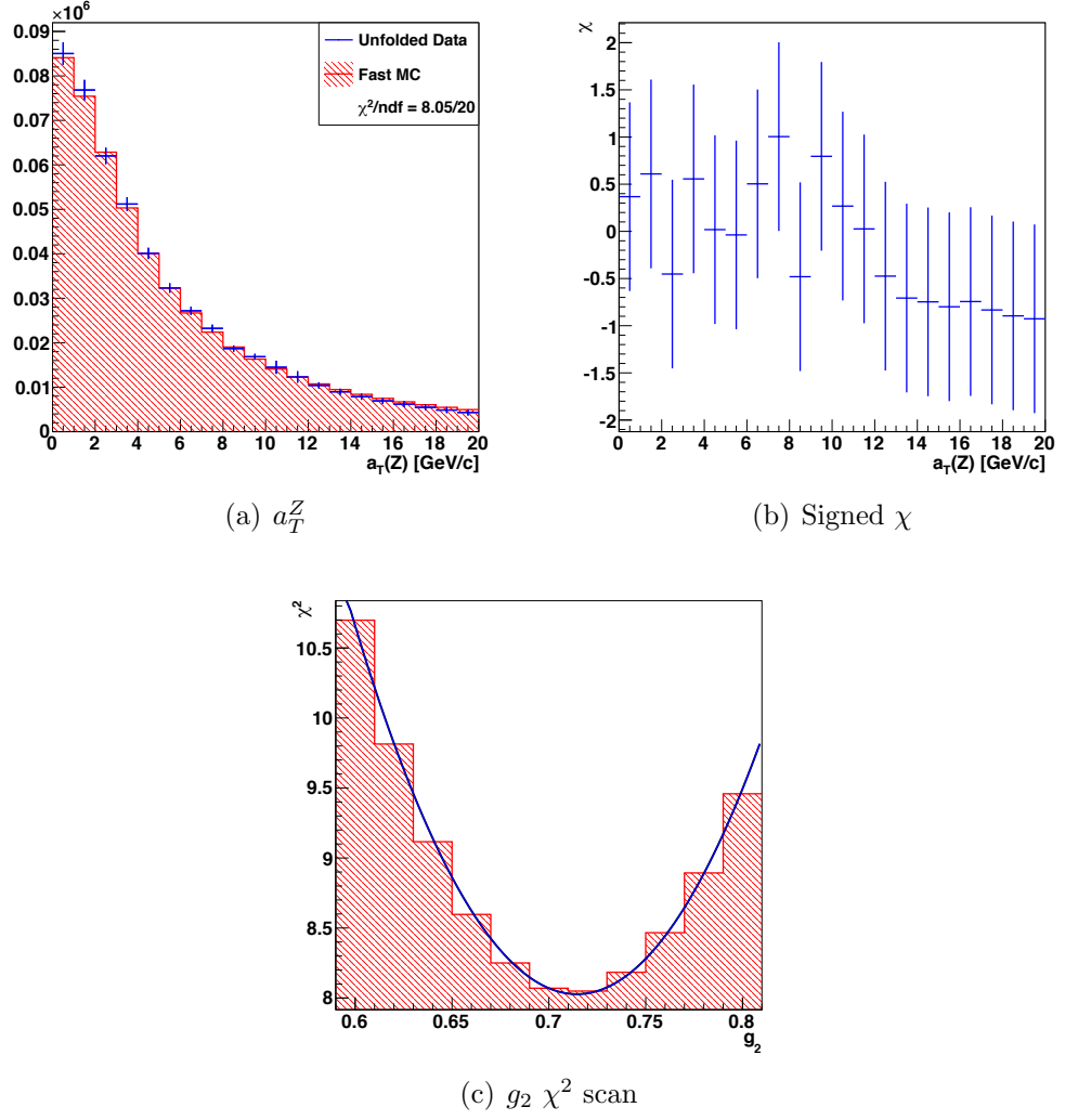
Figure 8.9: The best \chi^2 fit between the background subtracted and unfolded Z^0 \rightarrow e^+e^- data and g_2 -reweighted fast Monte Carlo. One iteration of the unfolding algorithm has been used to unfold the data.
