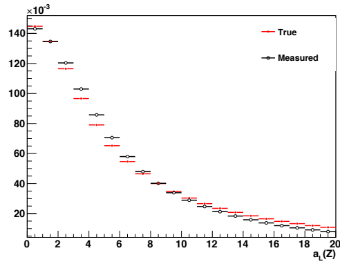
(c) a_L^Z
