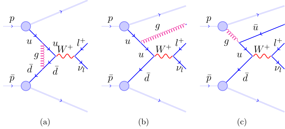
Figure 5.2: An example of W production and leptonic decay with next-to-leading order QCD effects.
