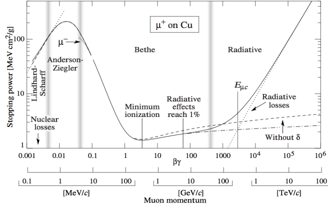
Figure 5.9: The stopping power, -\langle dE/dx \rangle , of copper for a muon over a large range of momentum. The muons from weak boson decays fall in the “Bethe” regime. [65]
