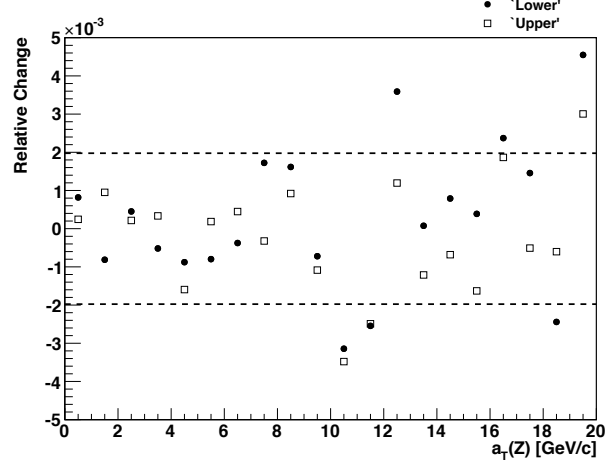
Figure 7.9: The relative error on an unfolded a_T^Z distribution incurred by adjusting the \kappa_{\text{CEM}} parameter by one standard deviation. The standard deviation of the shifts is marked by the dashed line.
