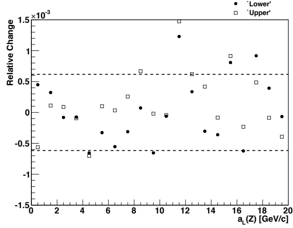
Figure 7.10: The relative error on an unfolded a_L^Z distribution incurred by adjusting the \kappa_{\text{CEM}} parameter by one standard deviation. The standard deviation of the shifts is marked by the dashed line.
