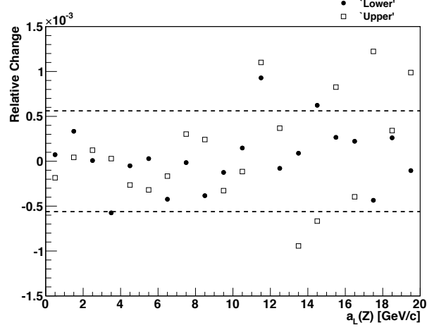
Figure 7.7: The relative error on an unfolded a_L^Z distribution incurred by adjusting the S_{\text{CEM}} parameter by one standard deviation. The standard deviation of the shifts is marked by the dashed line.
