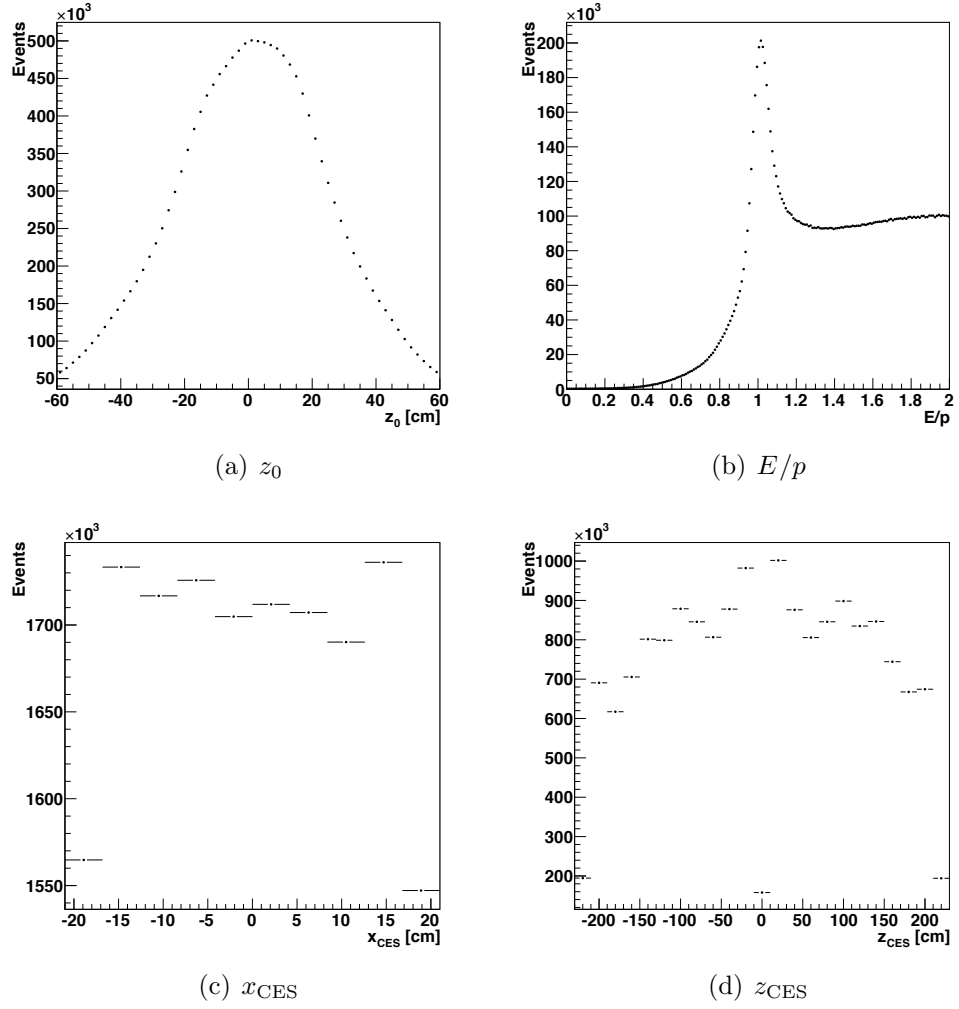
Figure 4.1: Cut variables for W \rightarrow e\nu data before cuts are applied. (a) The distribution of the primary interaction point, z_0 . (b) The E/p distribution has a peak at unity and the tail below unity that is produced by calorimeter resolution and energy leaking out of the calorimeter. The high tail above unity is caused by bremsstrahlung from the primary electron in the W decay. (c) The lower response at the edge of a calorimeter wedge is observed for |x_{CES}| > 18 cm. (d) The gap between calorimeter halves is observed for |z_{CES}| < 12 cm.
