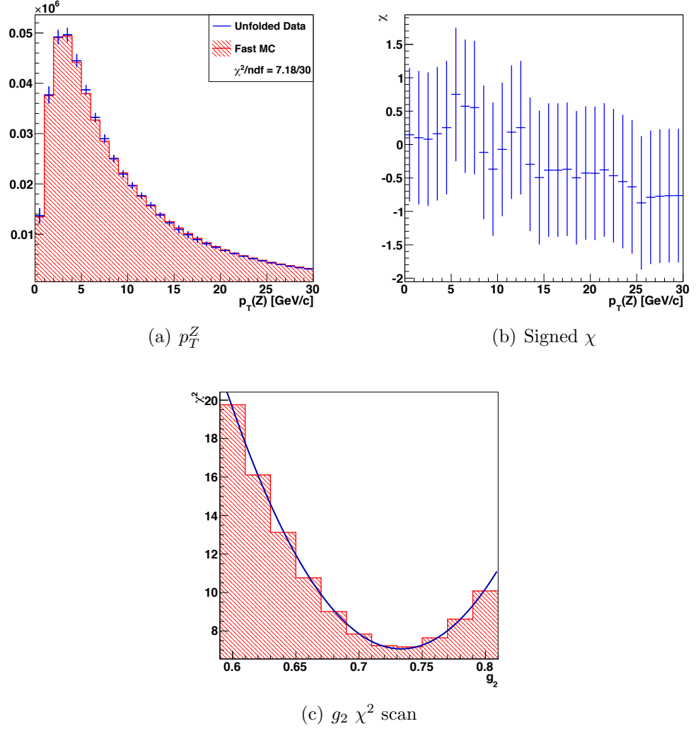
Figure 8.8: The best \chi^2 fit between the background subtracted and unfolded Z^0 \rightarrow e^+e^- data and g_2 -reweighted fast Monte Carlo. One iteration of the unfolding algorithm has been used to unfold the data.
