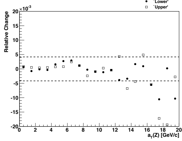
Figure 7.12: The relative error on an unfolded a_T^Z distribution incurred by adjusting the S_{\text{Mat}} parameter by one standard deviation. The standard deviation of the shifts is marked by the dashed line.
