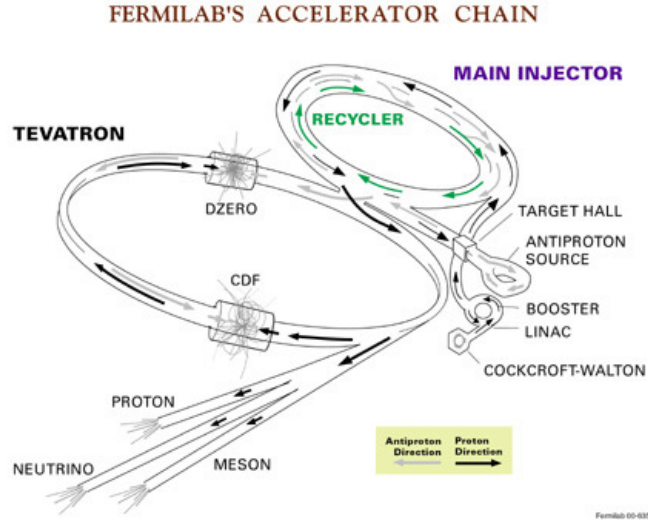
Figure 2.1: A schematic representation of the accelerator chain at Fermilab.
