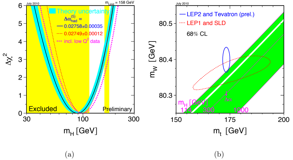
Figure 3.1: The standard model Higgs prediction from the recent LEP Electroweak Working group results [42, 43]. (a) The “blue band” plot showing the best fit value for the Higgs mass obtained using ZFITTER [44] with the LEP low-mass and Tevatron high-mass direct exclusions shown as shaded regions. (b) The constraint on a standard model Higgs boson from electroweak measurements. The contours show the 68% confidence intervals for direct (LEP2 and Tevatron) and indirect (LEP1 and SLD) measurements of the W and top quark masses. The diagonal stripe is the corresponding Higgs mass prediction. Unshaded regions of the plot are where a standard model Higgs has been excluded.
