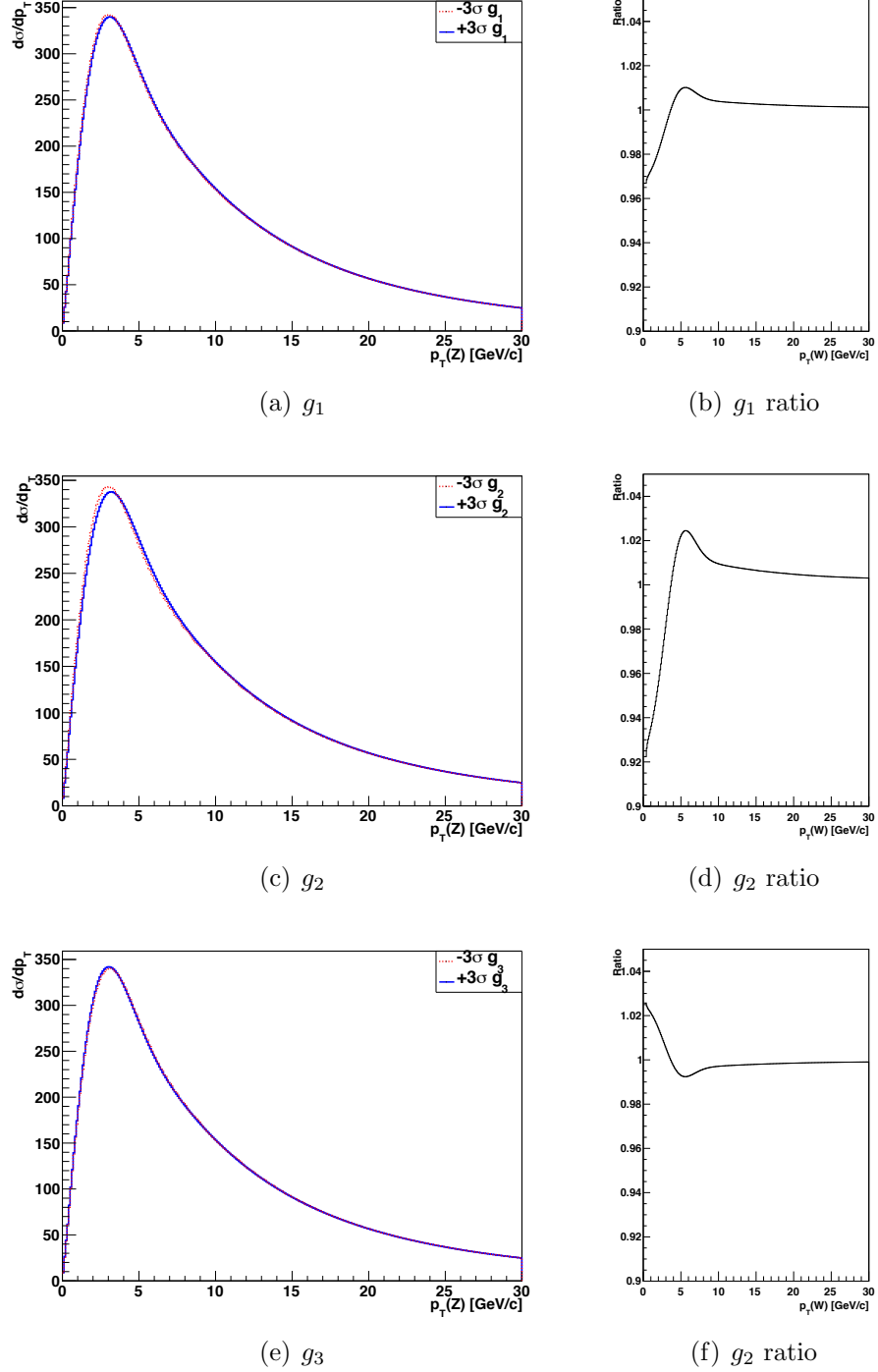
Figure 6.1: The change in d\sigma/dp_T by replacing g_i with g_i - 3\sigma and g_i + 3\sigma for each of the BLNY parameters. The global fit error in [60] is used for each parameter. The ratio between g_i - 3\sigma and g_i + 3\sigma shows the sensitivity of each g_i parameter.
