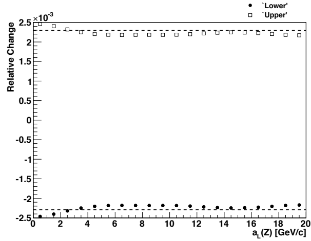
Figure 7.18: The relative error on an unfolded a_L^Z distribution incurred by adjusting the background fraction by one standard deviation. The standard deviation of the shifts is marked by the dashed line.
