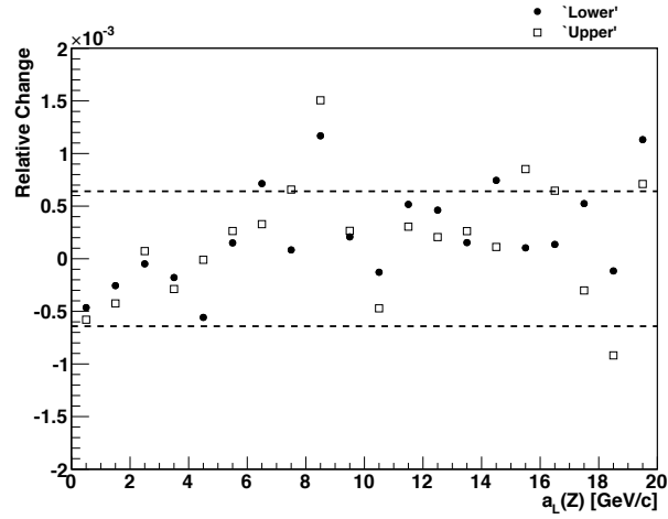
Figure 7.13: The relative error on an unfolded a_L^Z distribution incurred by adjusting the S_{\text{Mat}} parameter by one standard deviation. The standard deviation of the shifts is marked by the dashed line.
