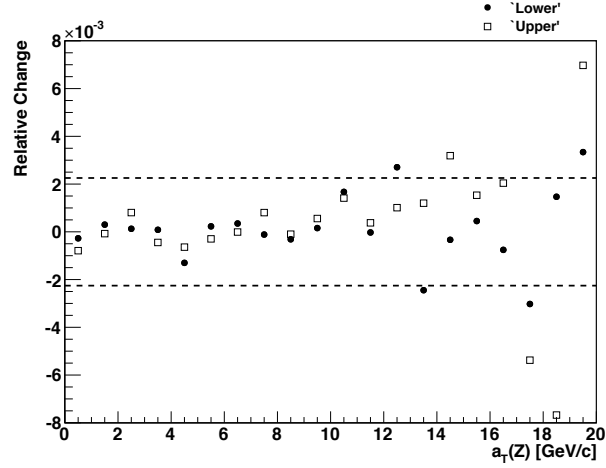
Figure 7.6: The relative error on an unfolded a_T^Z distribution incurred by adjusting the S_{\text{CEM}} parameter by one standard deviation. The standard deviation of the shifts is marked by the dashed line.
