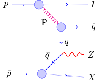
Figure 7.14: The diffractive production of Z^0 bosons. The proton emits a Pomeron, \mathbb{P} , and remains intact; the Pomeron decays into a quark-antiquark pair. The quark (antiquark) from the Pomeron annihilates with an antiquark (quark) from the antiproton.
