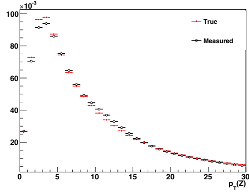
(a) p_T^Z
