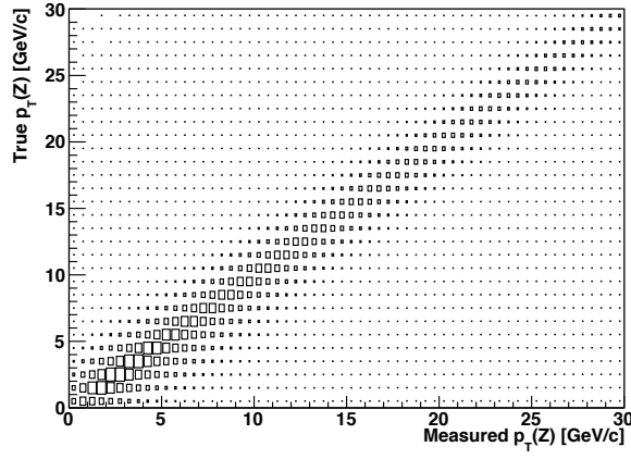
(a) p_T^Z
