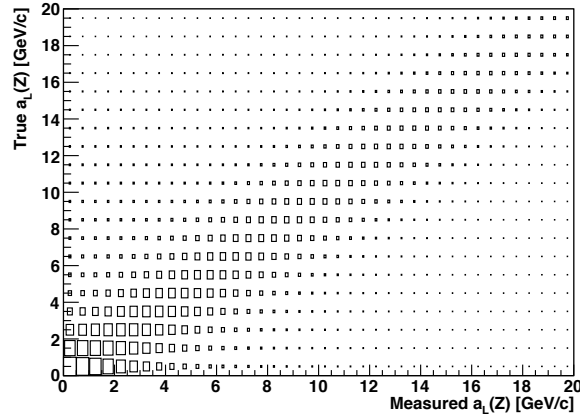
(c) a_L^Z
