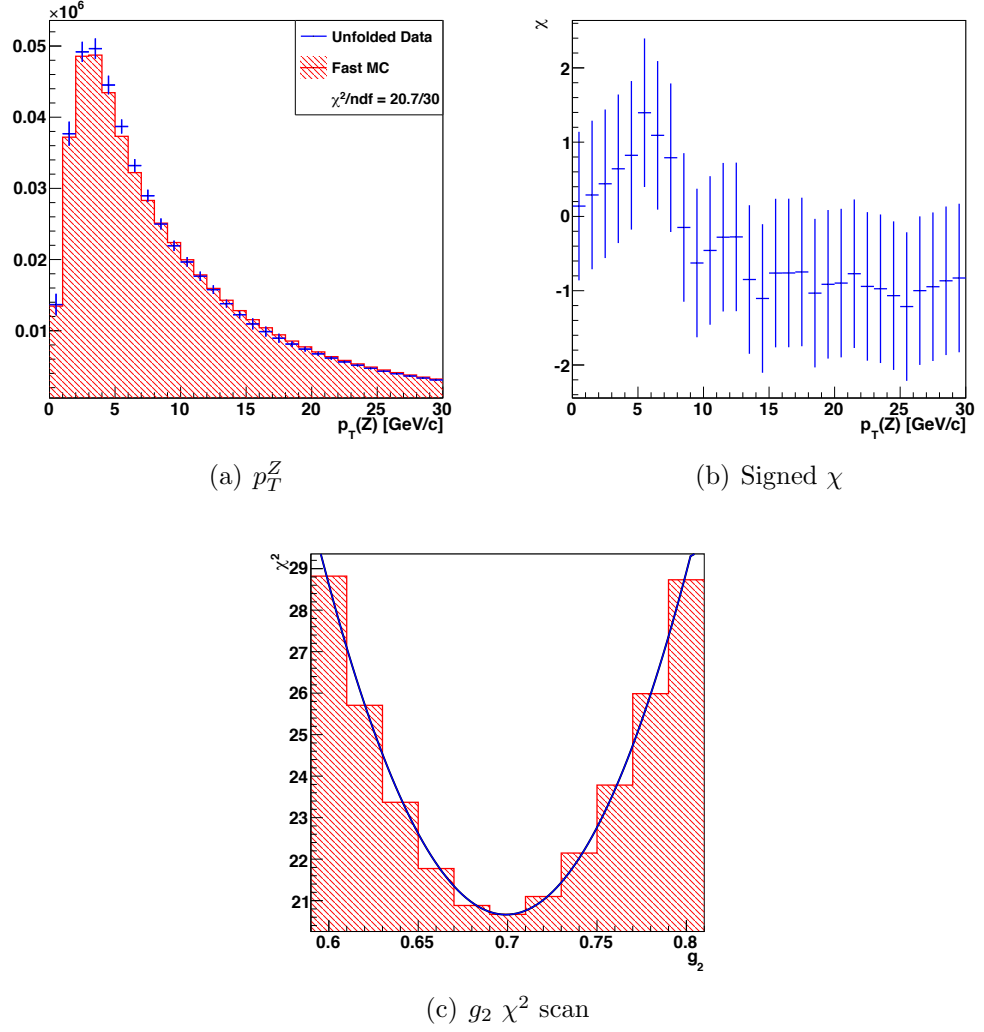
Figure 8.11: The best \chi^2 fit between the background subtracted and unfolded Z^0 \rightarrow e^+e^- data and g_2 -reweighted fast Monte Carlo using the KN global fit parameters for g_1 and g_3 . One iteration of the unfolding algorithm has been used to unfold the data.
