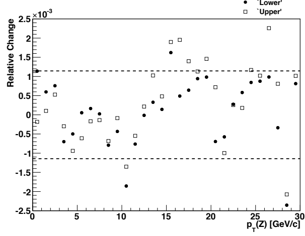
Figure 7.5: The relative error on an unfolded p_T^Z distribution incurred by adjusting the S_{\text{CEM}} parameter by one standard deviation. The standard deviation of the shifts is marked by the dashed line.
