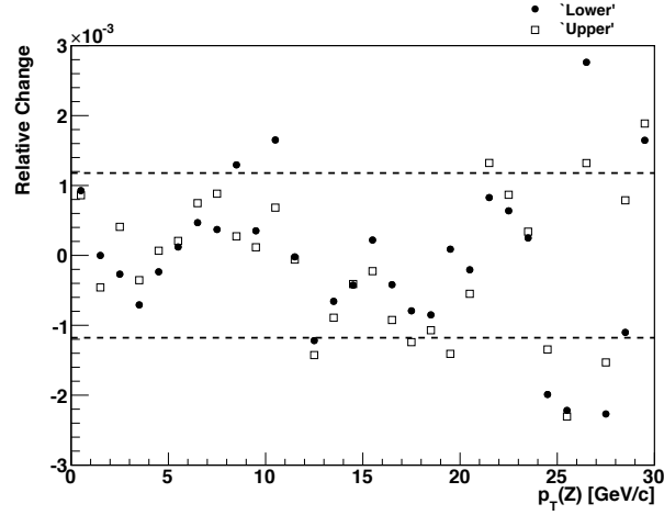
Figure 7.11: The relative error on an unfolded p_T^Z distribution incurred by adjusting the S_{\text{Mat}} parameter by one standard deviation. The standard deviation of the shifts is marked by the dashed line.
