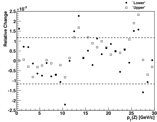
Figure 7.8: The relative error on an unfolded p_T^Z distribution incurred by adjusting the \kappa_{\text{CEM}} parameter by one standard deviation. The standard deviation of the shifts is marked by the dashed line.
