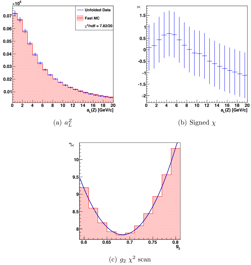
Figure 8.10: The best \chi^2 fit between the background subtracted and unfolded Z^0 \rightarrow e^+e^- data and g_2 -reweighted fast Monte Carlo. One iteration of the unfolding algorithm has been used to unfold the data.
