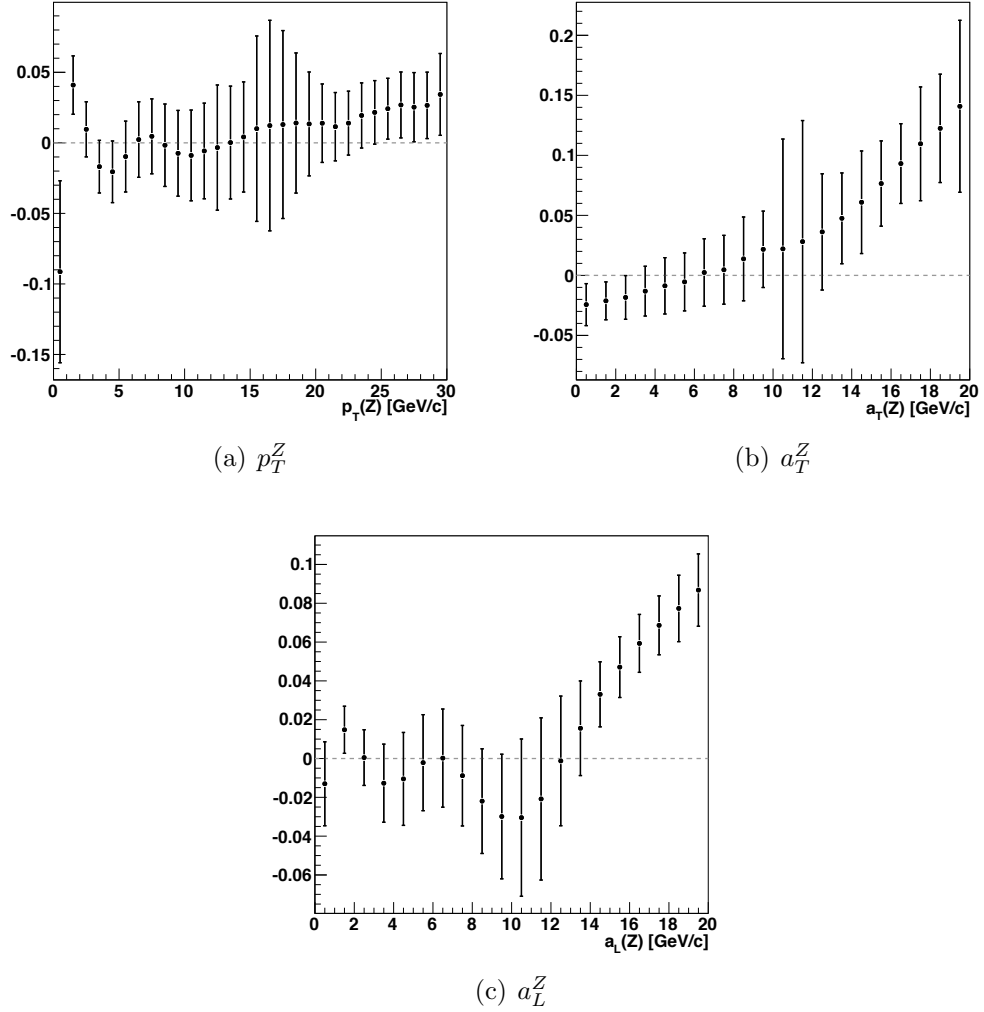
Figure 7.2: The mean and standard deviation of the shifts in each bin from the unfolding algorithm using 250 pseudo-experiments. \Delta_i , the relative shift in the i th bin is estimated for each pseudo-experiment where the mean \Delta_i is the systematic error induced by the algorithm in that bin and the standard deviation is the statistical error.
