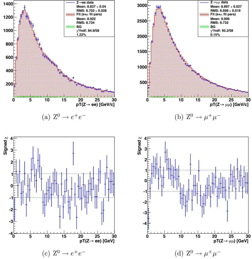
Figure 8.7: The best fit Monte Carlo compared against (a) Z^0 \rightarrow e^+e^- and (b) Z^0 \rightarrow \mu^+\mu^- data using g_2 = 0.623 \text{ GeV}^2 and with \xi fixed at 0.1201 (PDF set value). The signed \chi distributions are also shown for (c) Z^0 \rightarrow e^+e^- and (d) Z^0 \rightarrow \mu^+\mu^- .
