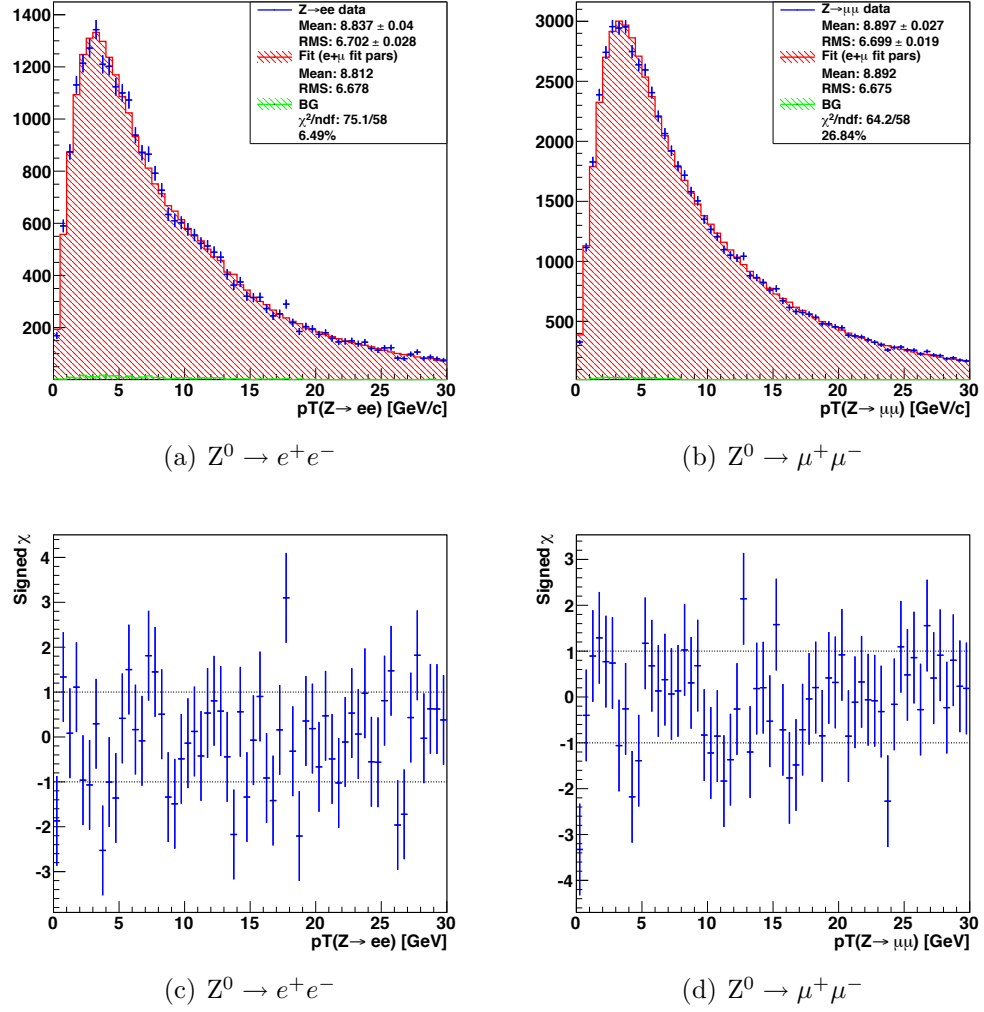
Figure 8.6: The best fit Monte Carlo compared against (a) Z^0 \rightarrow e^+e^- and (b) Z^0 \rightarrow \mu^+\mu^- data using g_2 = 0.721 \text{ GeV}^2 and \xi = 0.1167 . The signed \chi distributions are also shown for (c) Z^0 \rightarrow e^+e^- and (d) Z^0 \rightarrow \mu^+\mu^- .
