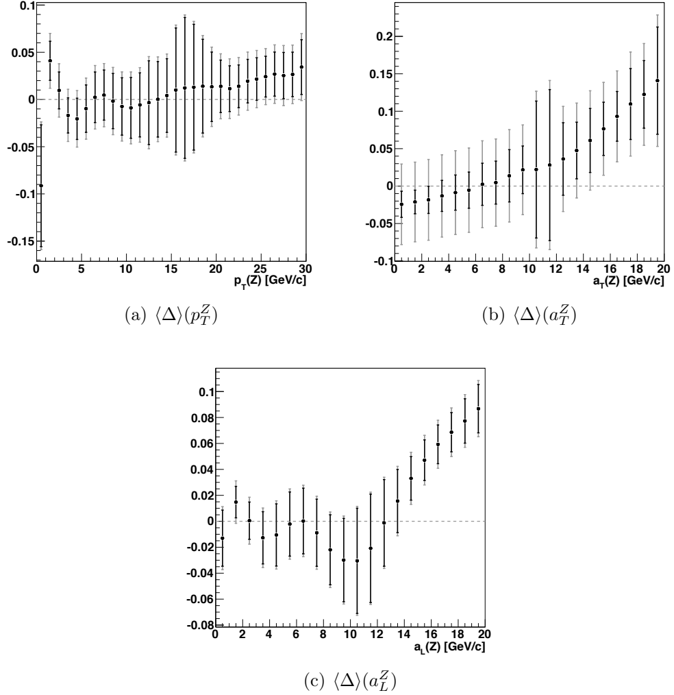
Figure 7.20: The statistical uncertainty of the unfolding method on the unfolded distributions is shown with the systematic shift of the unfolding method. The additional error bar shows the contribution of the CEM and material scale systematic uncertainties and the background fraction uncertainty all scaled by a factor of 10 and added in quadrature.
