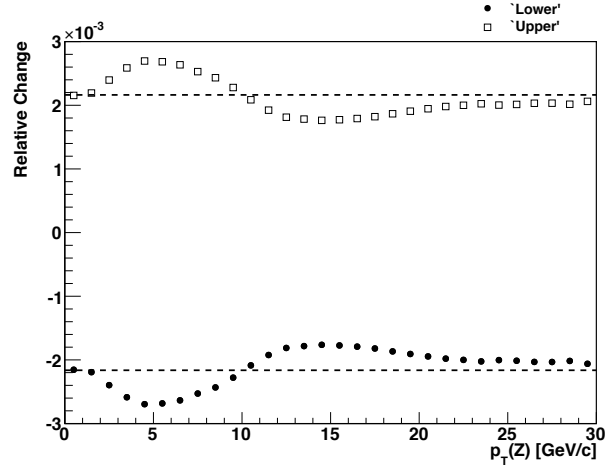
Figure 7.16: The relative error on an unfolded p_T^Z distribution incurred by adjusting the background fraction by one standard deviation. The standard deviation of the shifts is marked by the dashed line.
