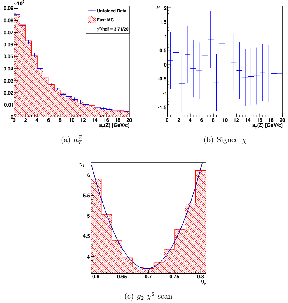
Figure 8.12: The best \chi^2 fit between the background subtracted and unfolded Z^0 \rightarrow e^+e^- data and g_2 -reweighted fast Monte Carlo using the KN global fit parameters for g_1 and g_3 . One iteration of the unfolding algorithm has been used to unfold the data.
