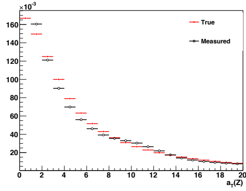
(b) a_T^Z
