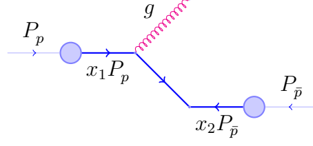
Figure 3.3: The centre-of-mass energy system for a quark and antiquark emitted from a head-on collision between parallel proton and antiproton beams with initial state gluon emission. The gluon emitted prior to the quark-antiquark interaction imparts some net transverse momentum on the quark-antiquark system.
