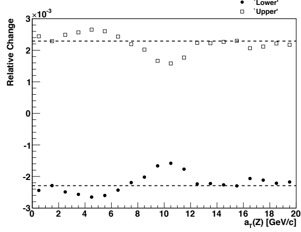
Figure 7.17: The relative error on an unfolded a_T^Z distribution incurred by adjusting the background fraction by one standard deviation. The standard deviation of the shifts is marked by the dashed line.
