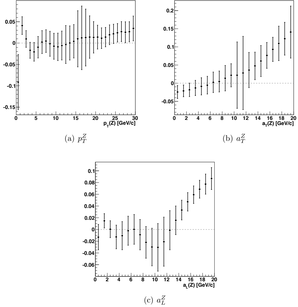
Figure 7.19: The statistical uncertainty of the unfolding method on the unfolded distributions is shown with the systematic shift of the unfolding method. The additional error bar shows the contribution of the CEM and material scale systematic uncertainties and the background fraction uncertainty added in quadrature.
