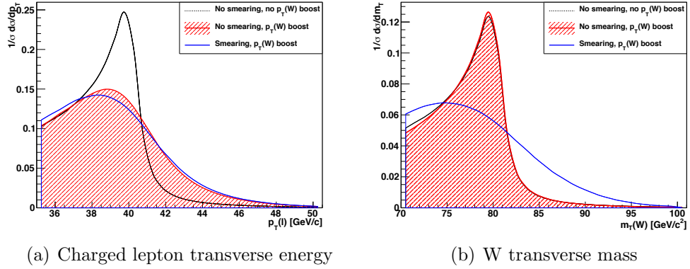
Figure 3.4: The effect of the the W transverse momentum, |\mathbf{p}_T^W| , on the Jacobian edge for (a) the charged lepton transverse energy and (b) the transverse mass of the W. The dotted line is the variable in the lab frame before simulating detector resolution or acceptance for |\mathbf{p}_T^W| = 0 . The shaded area is the variable in the lab frame before simulating detector resolution or acceptance for |\mathbf{p}_T^W| \neq 0 . The solid line is the variable in the lab frame after simulating detector resolution and acceptance for |\mathbf{p}_T^W| \neq 0 .
