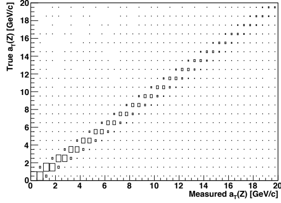
(b) a_T^Z
