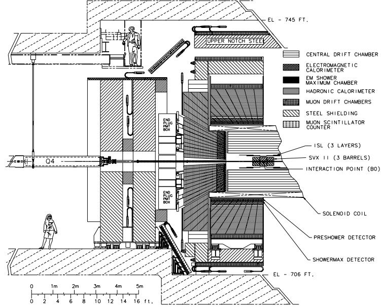
Figure 2.4: An elevation view of half of CDF showing the various detector subsystems.
