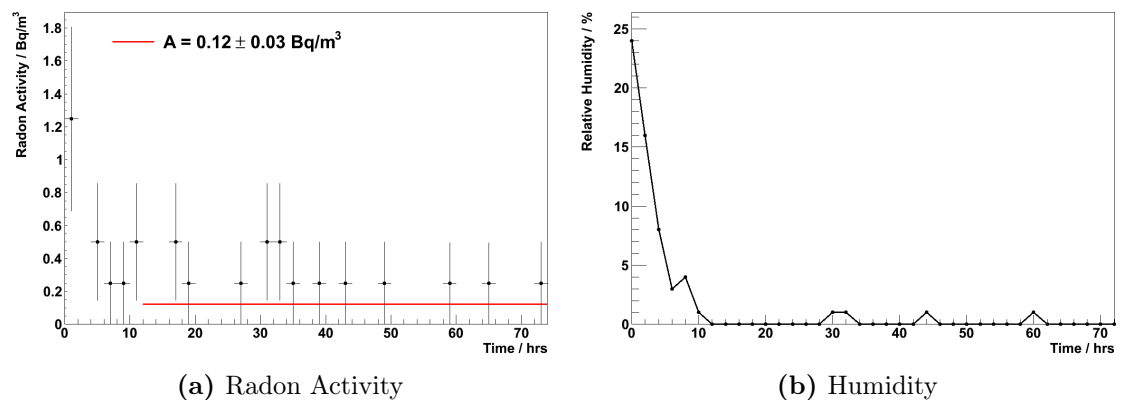
Figure 7.12: Measurements made by the RAD7 device inside the anti-radon tent during a C-section measurement. Radon activity and humidity measurements are shown.
