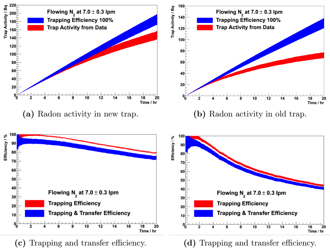
Figure 6.22: Comparison of trapping and trapping/transfer efficiencies of the new (plots a and c) and old (plots b and d) carbon trap.
