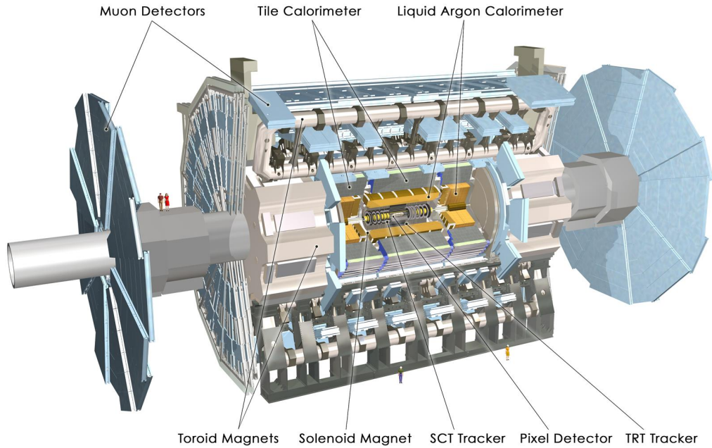
Figure 2.1.: A diagram of the ATLAS detector [28].
