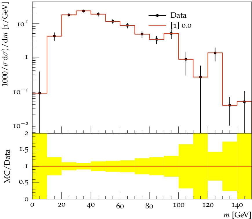
Filtered AK7 Z+jets, p_{T,j} = 300\text{--}450 GeV
