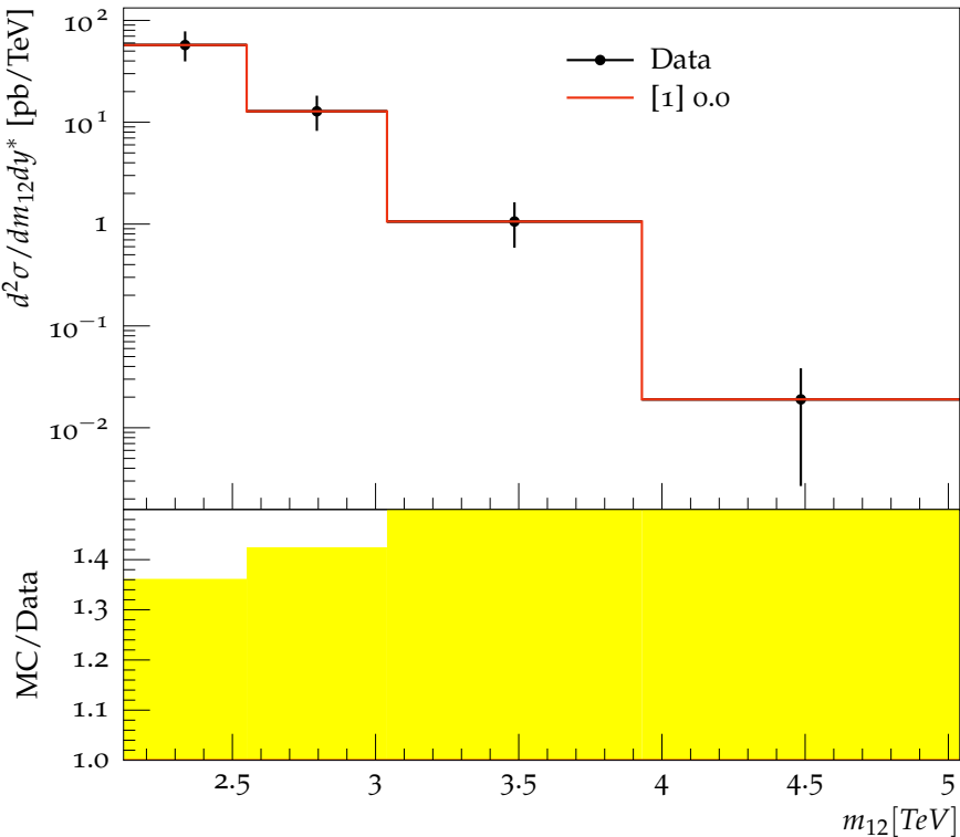
Dijet double-differential cross sections ( 2.5 < y^* < 3.0 ), R=0.4
