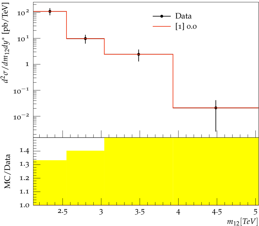
Dijet double-differential cross sections ( 2.5 < y^* < 3.0 ), R=0.6
