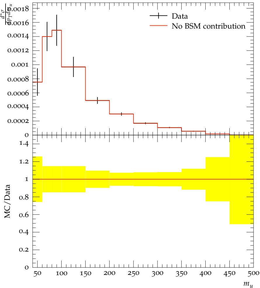
CMS, 13 TeV, Ungroomed jet mass m_u ( 900 < p_T < 1000 GeV)
