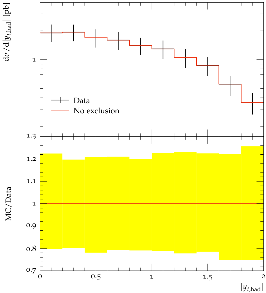
Combined lepton channels, boosted
