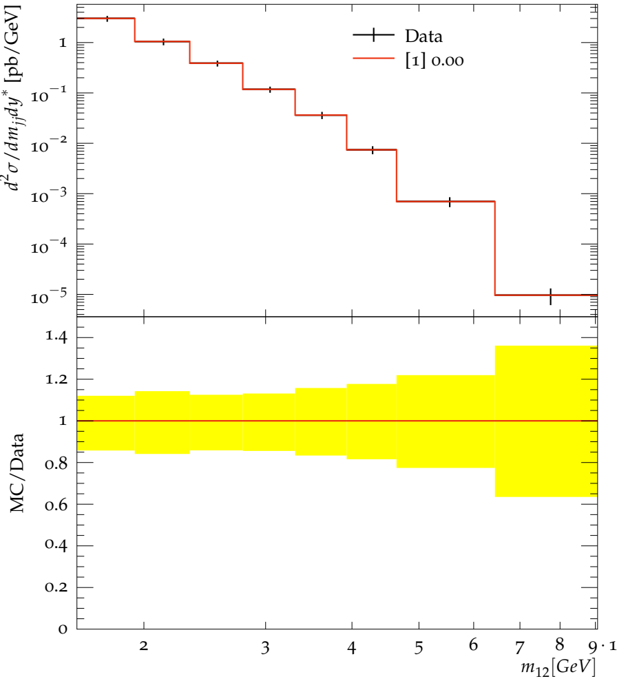
Dijet cross section ( 2.5 \leq y^* < 3.0 ), R=0.4
