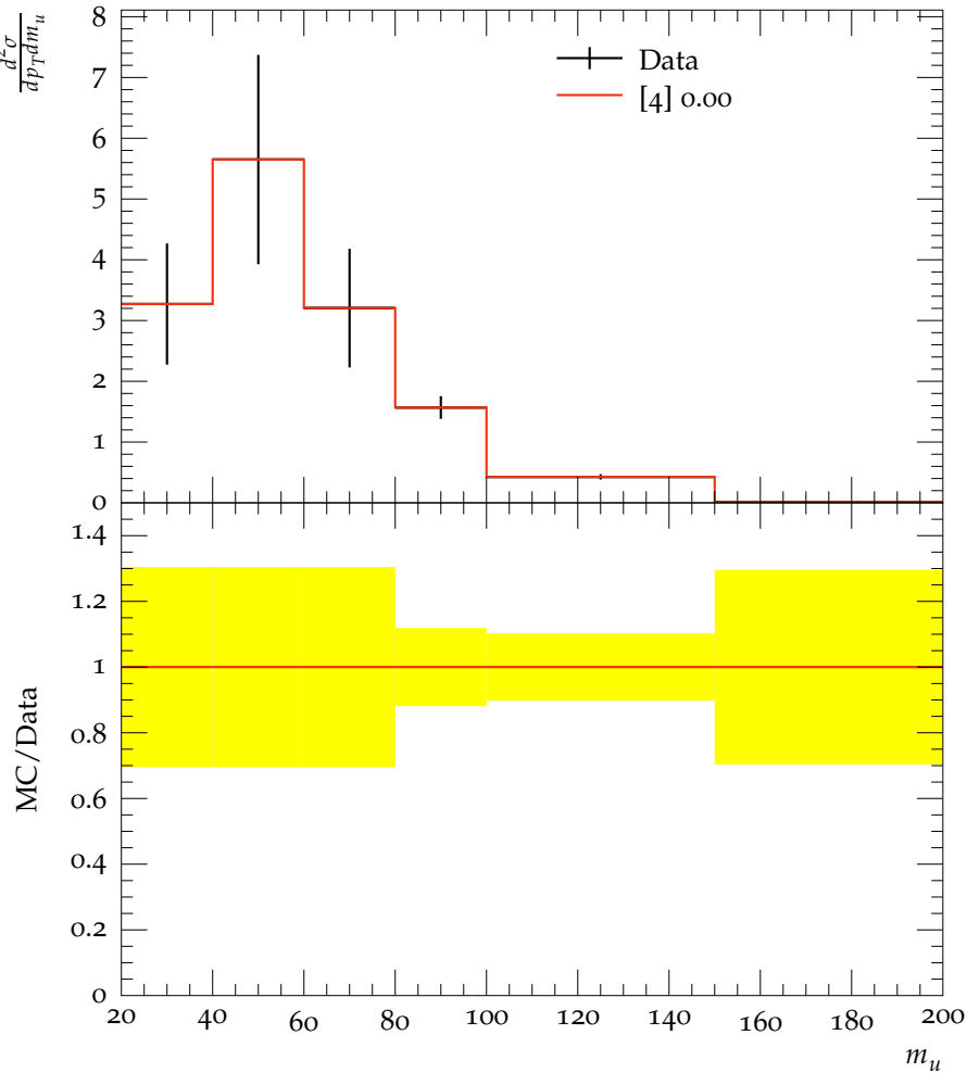
CMS, 13 TeV, Ungroomed jet mass m_u ( 260 < p_T < 350 GeV)
