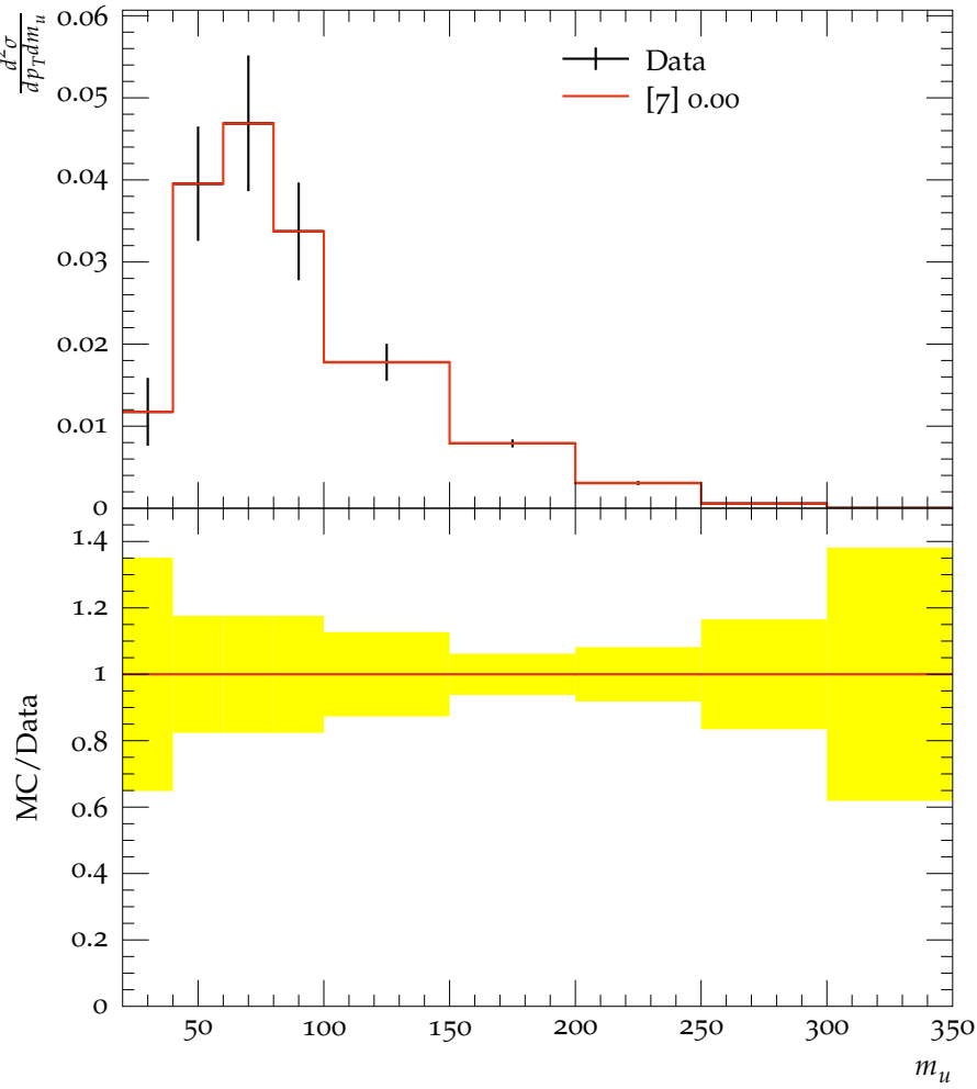
CMS, 13 TeV, Ungroomed jet mass m_u ( 550 < p_T < 650 GeV)
