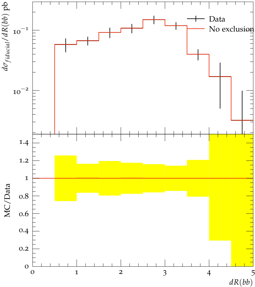
CMS, 8 TeV, DeltaR bb, at least two b jets
