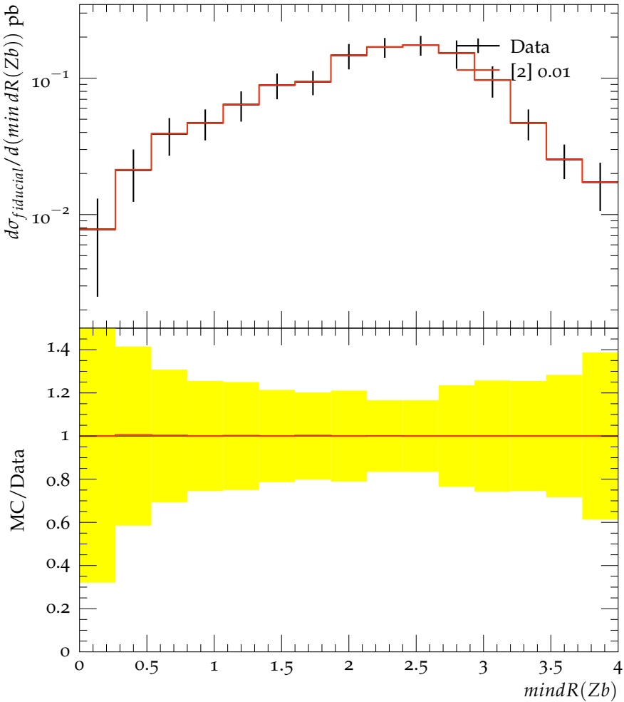
CMS, 8 TeV, DeltaR Zb minimum, at least two b jets
