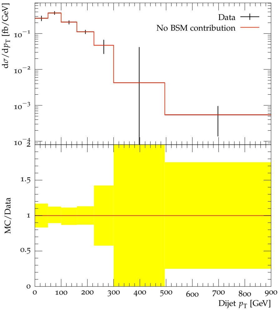
QCD+EW Wjj inclusive region with M_{jj} > 1.5 TeV: W \rightarrow \ell\nu
