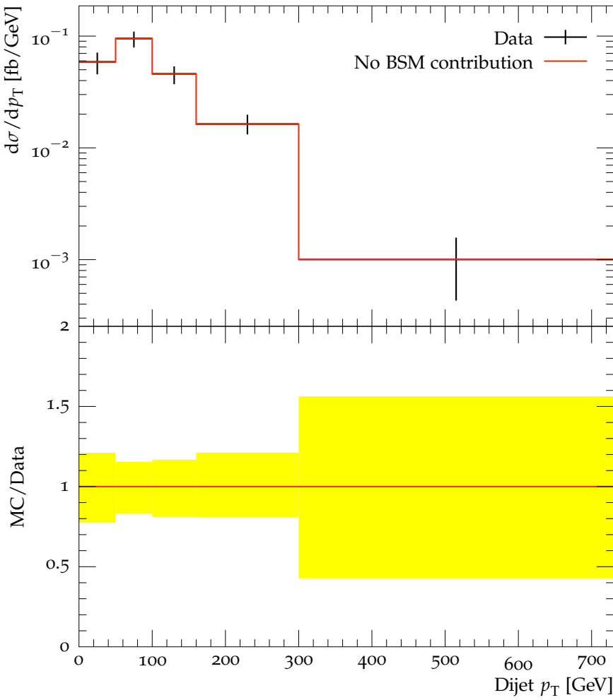
QCD+EW Wjj inclusive region with M_{jj} > 2.0 TeV: W \rightarrow \ell\nu
