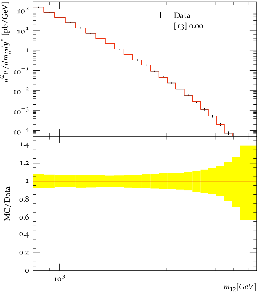
Dijet cross section ( 1.5 \leq y^* < 2.0 ), R=0.4
