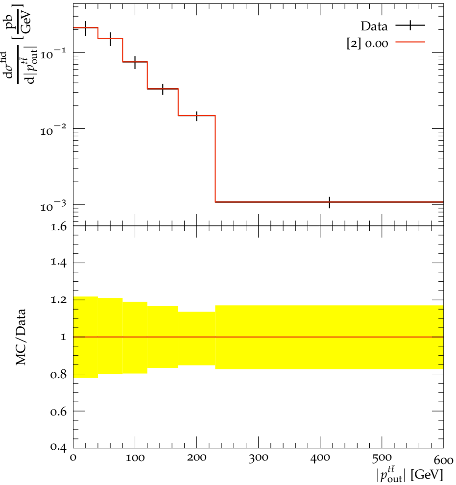
combined lepton channels, 6jizbi
