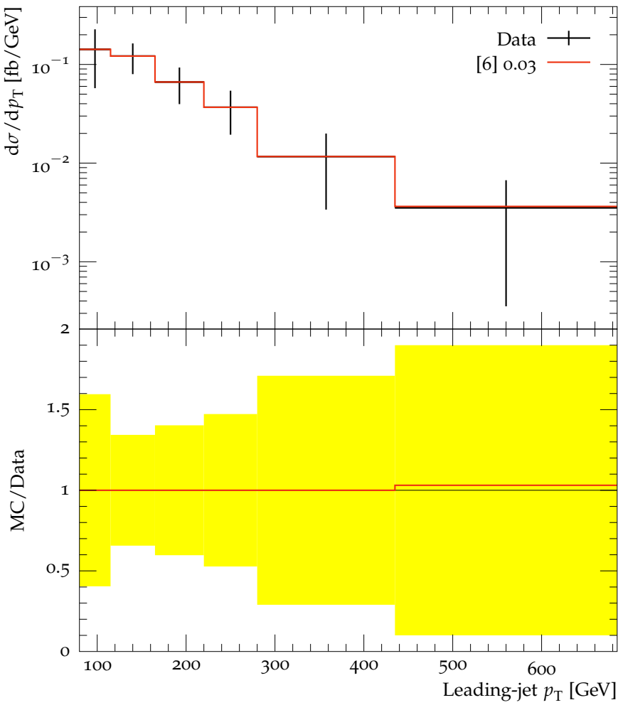
EW-only Wjj inclusive region with M_{jj} > 1.5 TeV: W \rightarrow \ell\nu
