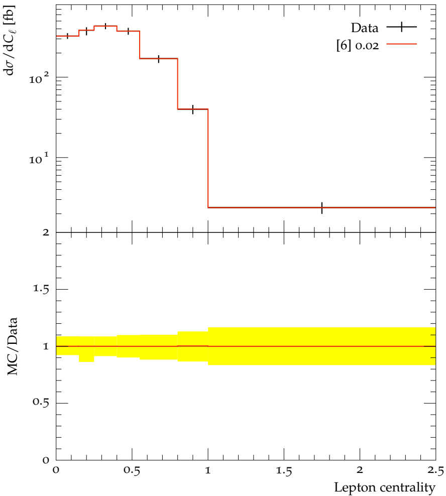
QCD+EW Wjj inclusive region with M_{jj} > 1.0 TeV: W \rightarrow \ell\nu
