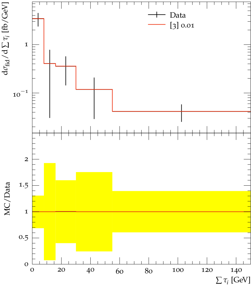
Sum of beam-thrust-like variables for jets, N_{jet} \geq 0, p_T^{jet} > 25 GeV
