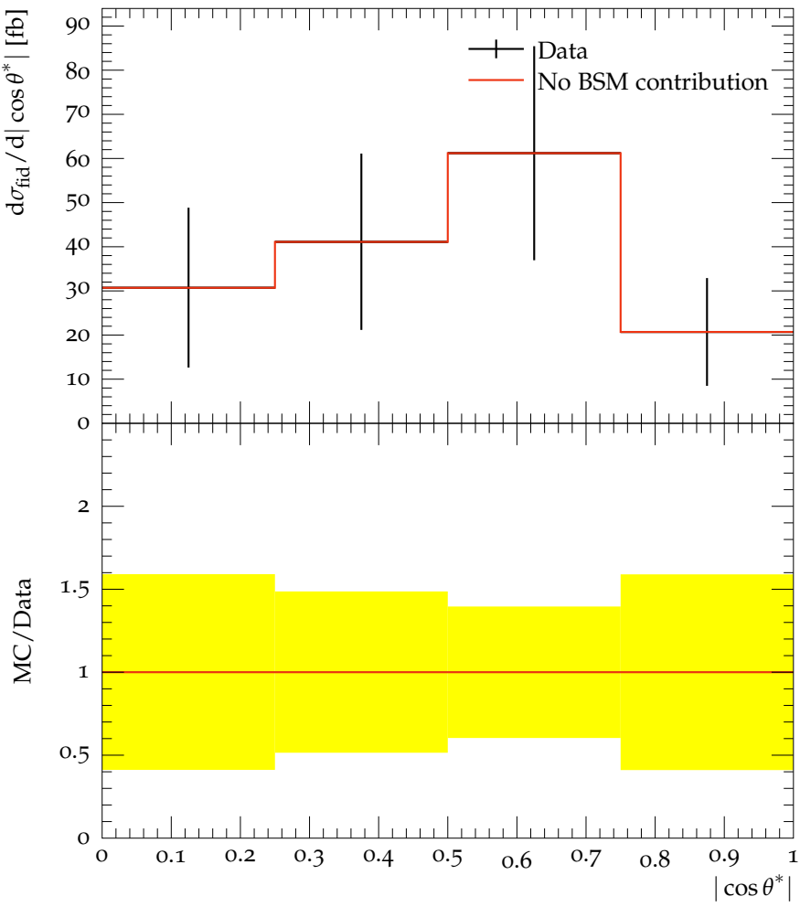
Photon decay angle in the Collins-Soper frame, p_T^{\gamma\gamma} < 80 GeV
