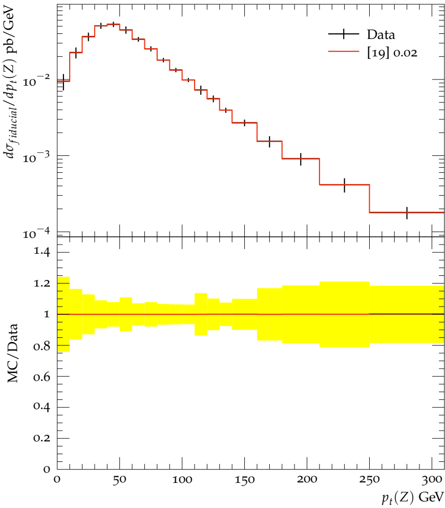
CMS, 8 TeV, Z boson pt, at least one b jet
