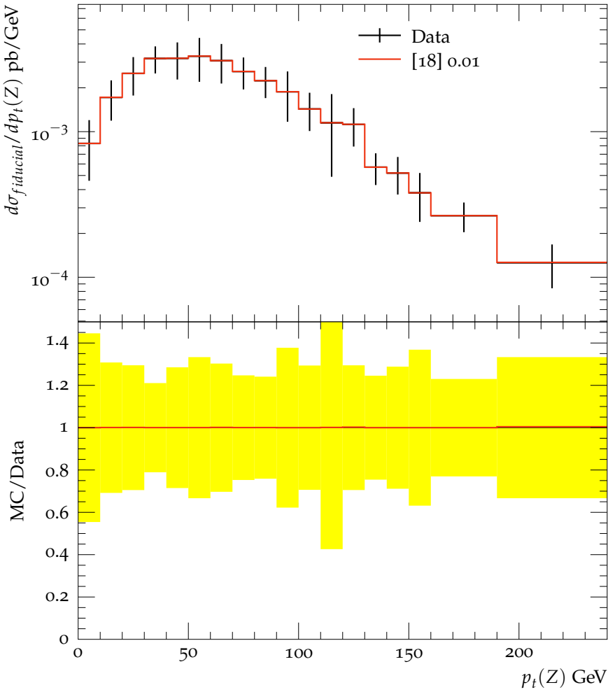
CMS, 8 TeV, Z boson pt, at least two b jets
