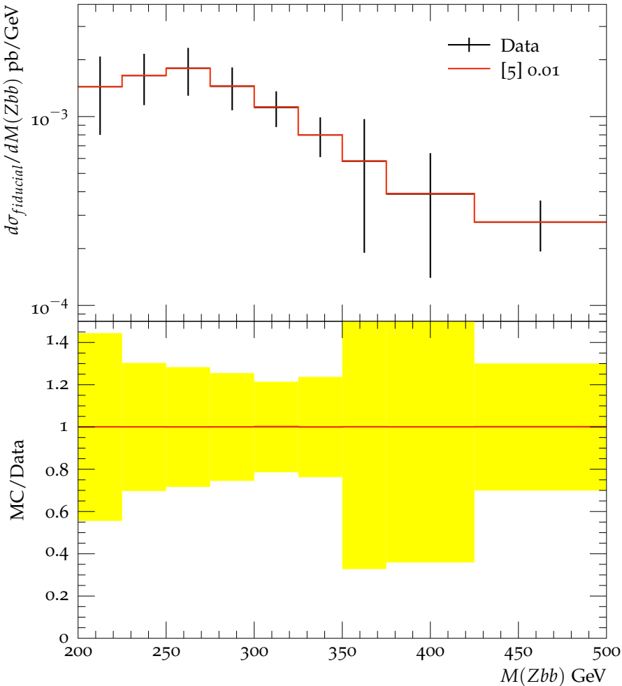
CMS, 8 TeV, Zbb system mass, at least two b jets
