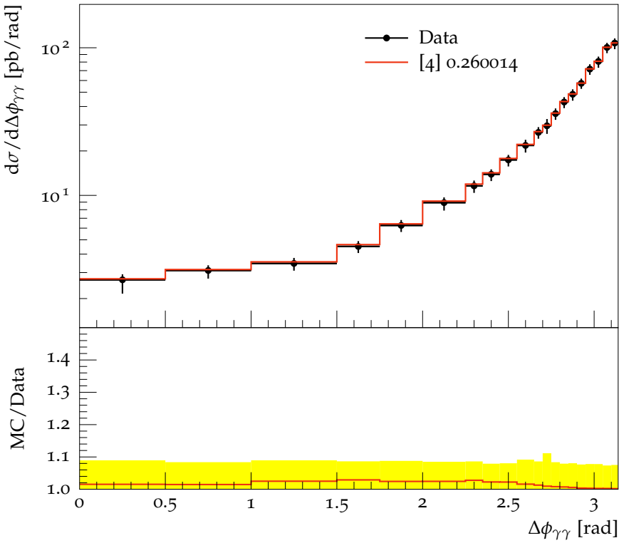
Isolated diphoton cross-section vs diphoton azimuthal separation
