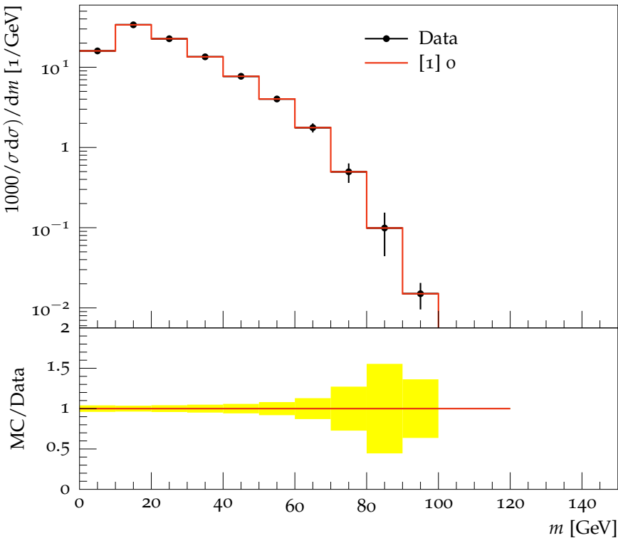
Trimmed AK7 W+jets, p_{T,j} = 150\text{--}220 GeV
