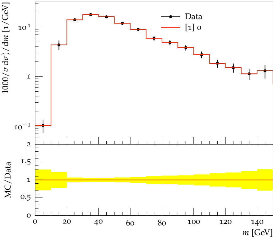
Filtered CA12 W+jets, p_{T,j} = 300\text{--}450 GeV
