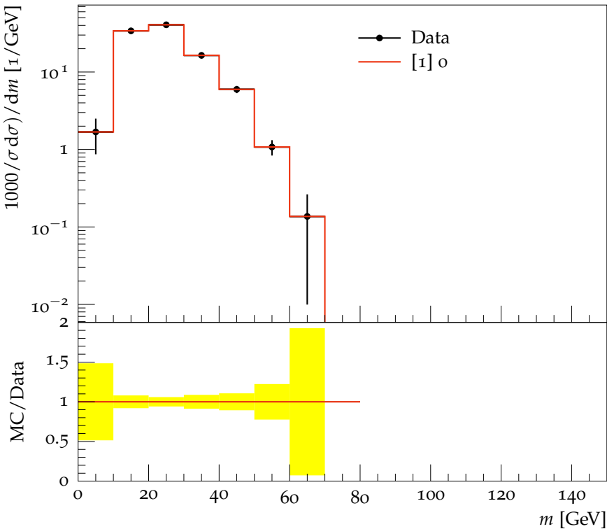
Filtered AK7 Z+jets, p_{T,j} = 125-150 GeV
