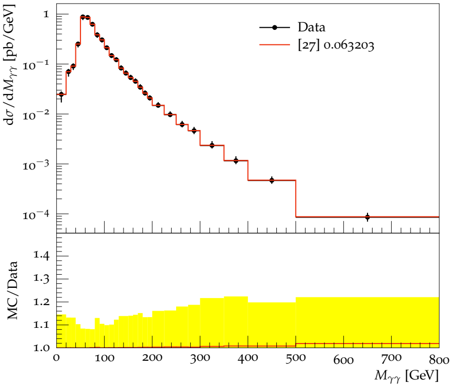
Isolated diphoton cross-section vs diphoton invariant mass
