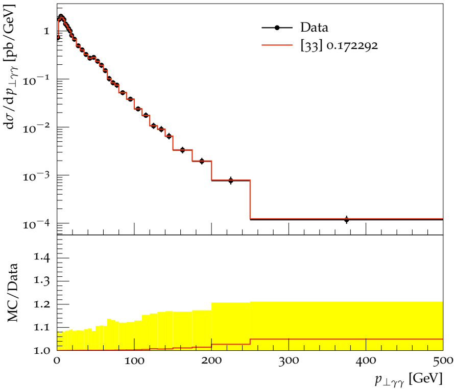
Isolated diphoton cross-section vs diphoton transverse momentum
