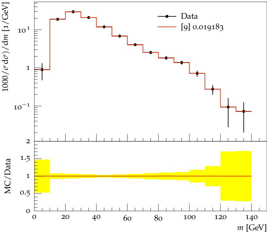
Filtered CA12 W+jets, p_{T,j} = 150\text{--}220 GeV
