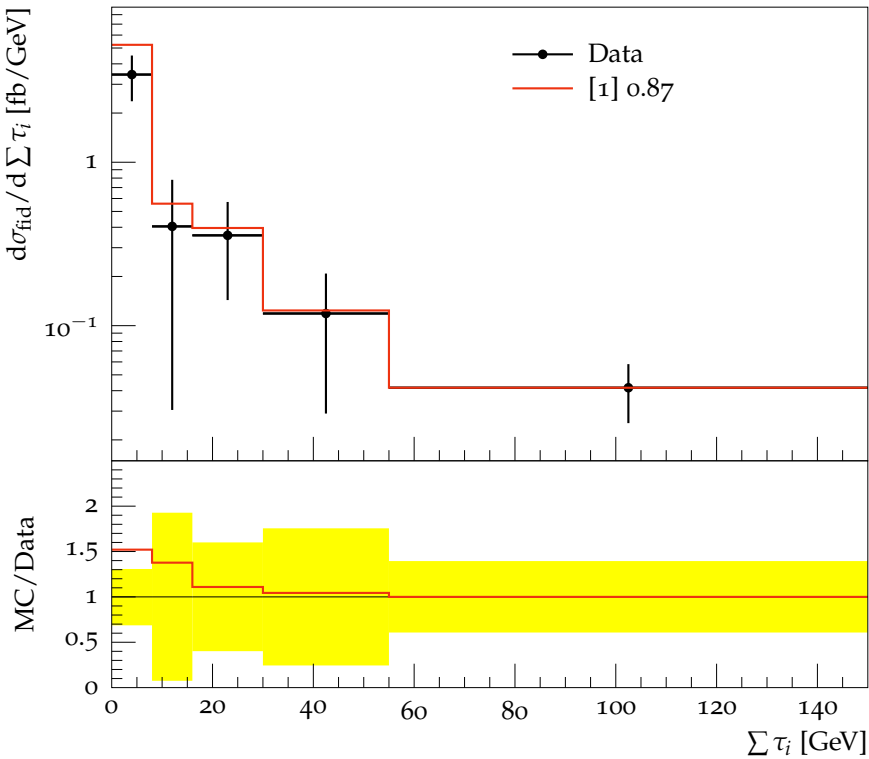
Sum of beam-thrust-like variables for jets, N_{jet} \geq 0, p_T^{jet} > 25 GeV
