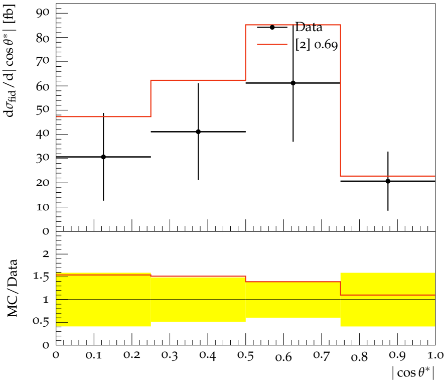
Photon decay angle in the Collins-Soper frame, p_T^{\gamma\gamma} < 80 GeV
