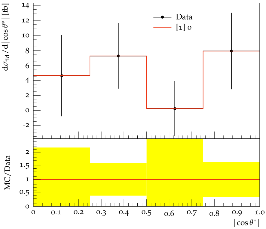
Photon decay angle in the Collins-Soper frame, 80 < p_T^{\gamma\gamma} < 200 Ge
