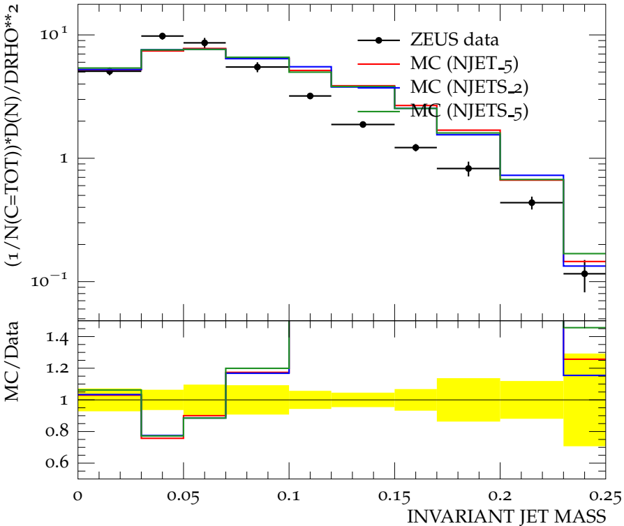
A Differential Distribution of Invariant Jet Mass
