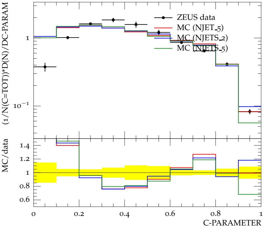
A Differential Distribution of the C-Parameter
