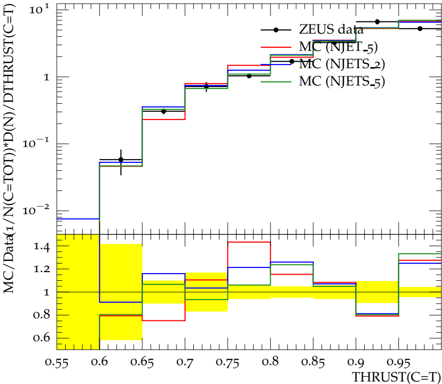
Differential Distribution of Thrust Relative to the Thrust Axis
