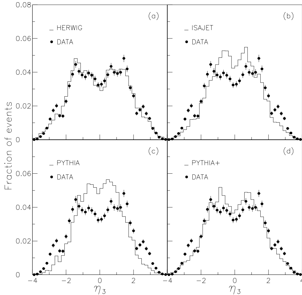
Figure 10: Observed \eta_3 distribution compared to the predictions of: (a) HERWIG; (b) ISAJET; (c) PYTHIA; (d) PYTHIA+.
