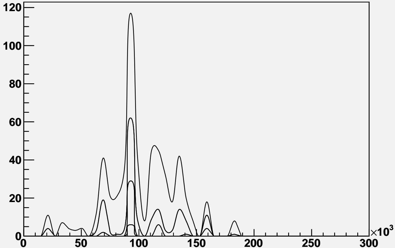
Dijet mass spectra of first two subjects, per p_T cut value
