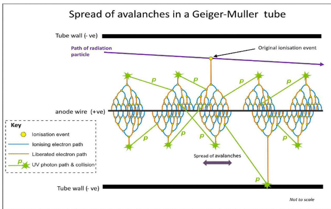
Figure 3.5: GeigerMechanismtrum [40]
