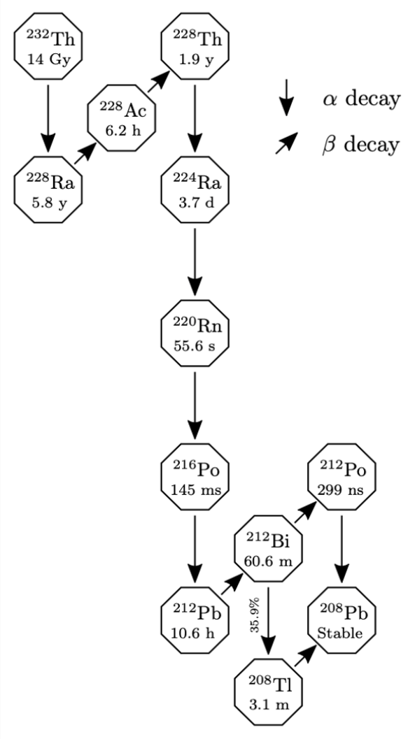
Figure 3.13: Tl208DecayScheme
