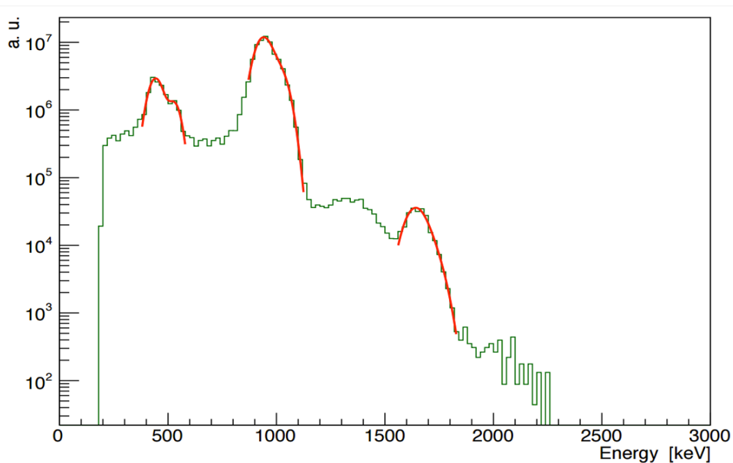
Figure 3.7: 207 Bi Spectrum
