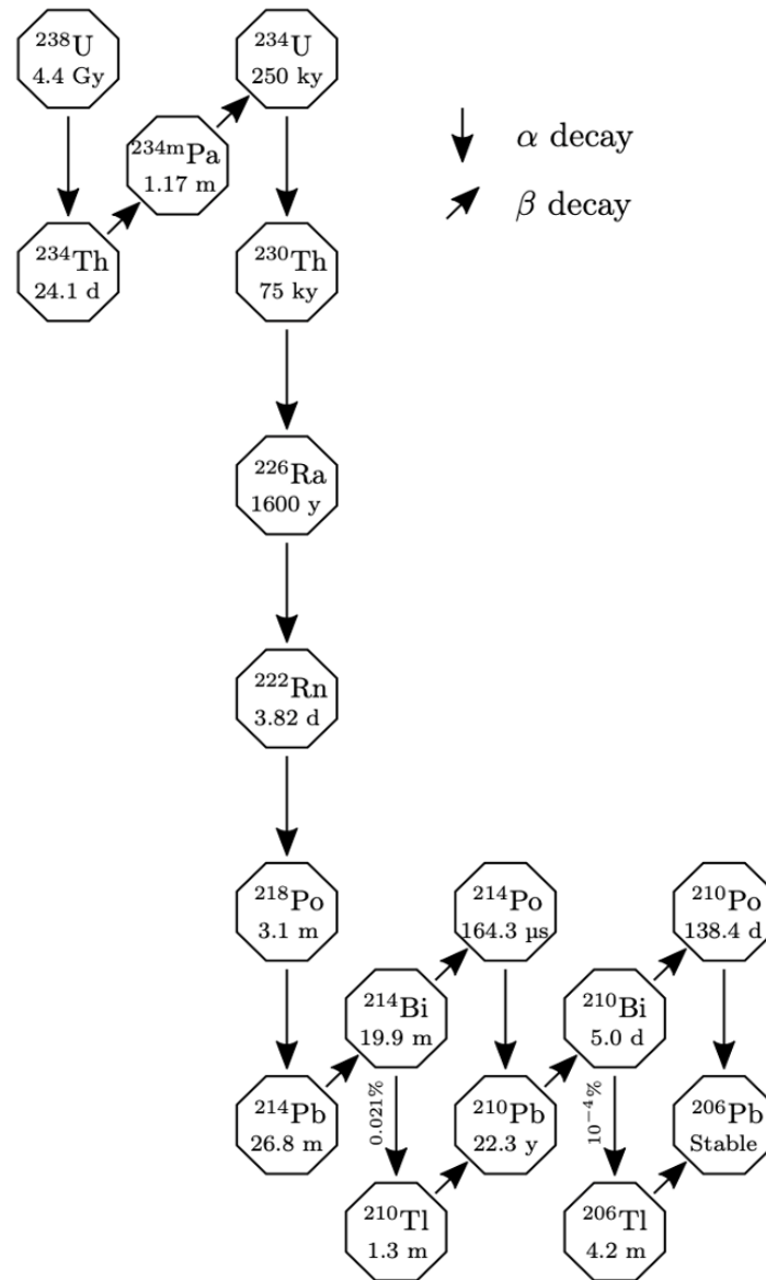
Figure 3.12: Bi214DecayScheme
