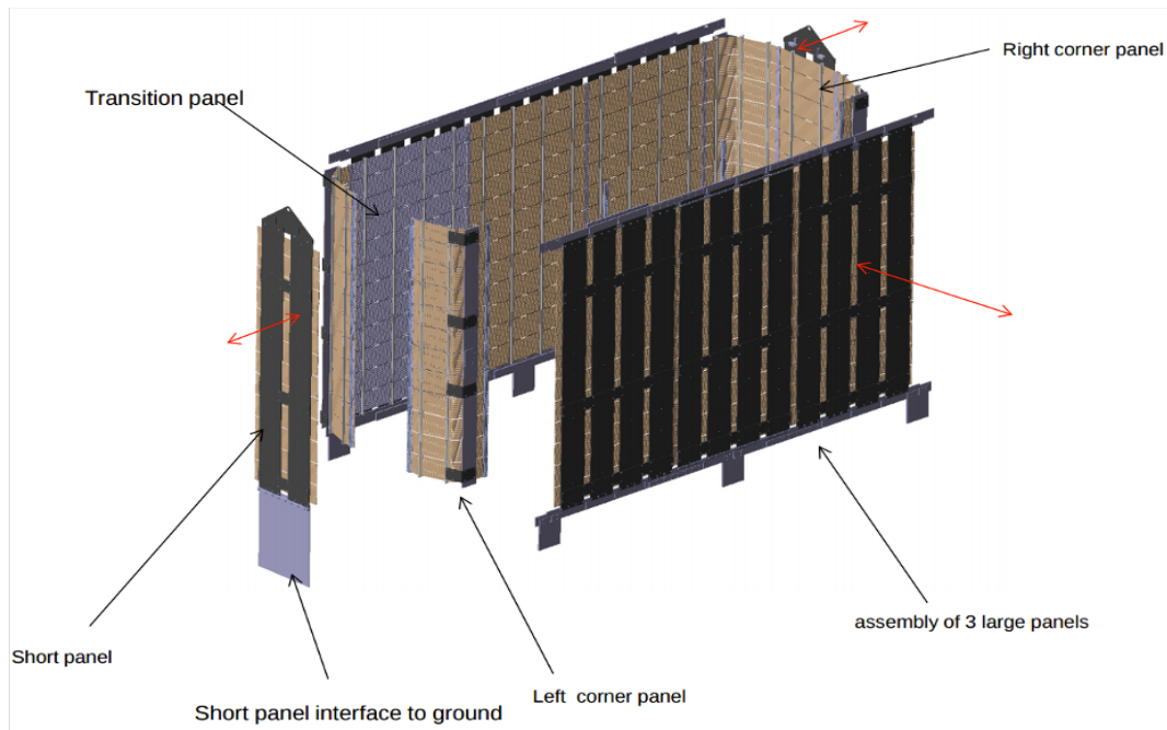
Figure 3.15: Open view of the magnetic coil illustrating the key components of the structure.
