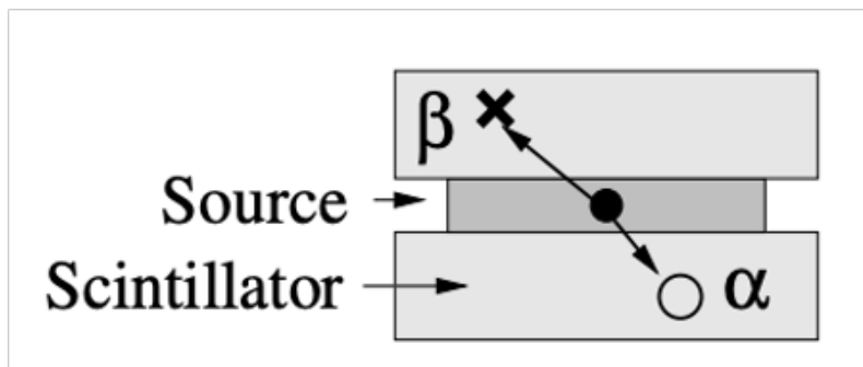
Figure 3.11: BiPoDetector [101]
