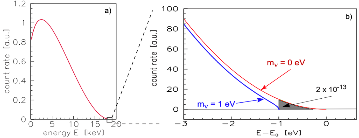
Figure 1.3: BetaSpectrum [11]
