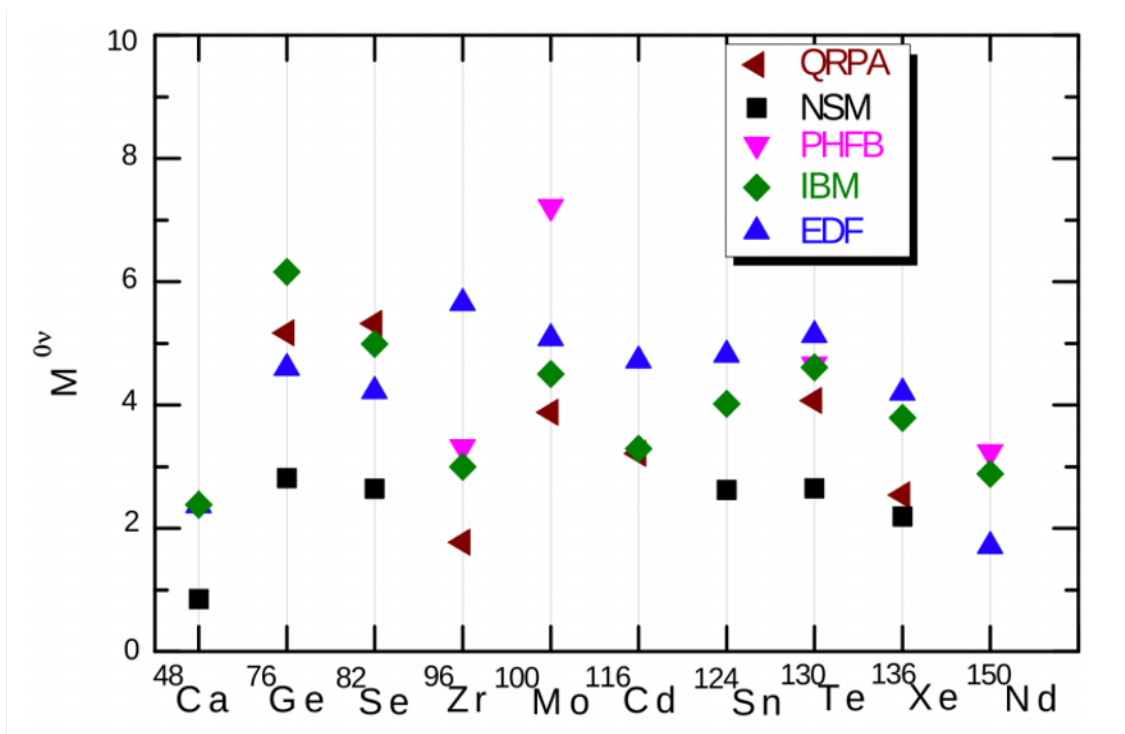
Figure 2.10: Nuclear matrix element (NME) values for the main double beta decaying isotopes used for experimentation, using the different methods described in Section 2.4 [35].
