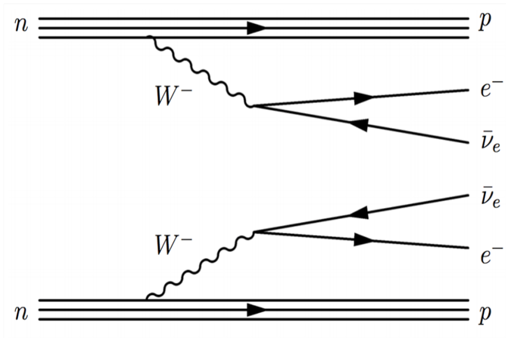
Figure 2.2: Feynman diagram for the Standard Model two neutrino double beta decay ( 2\nu\beta\beta ) [16].
