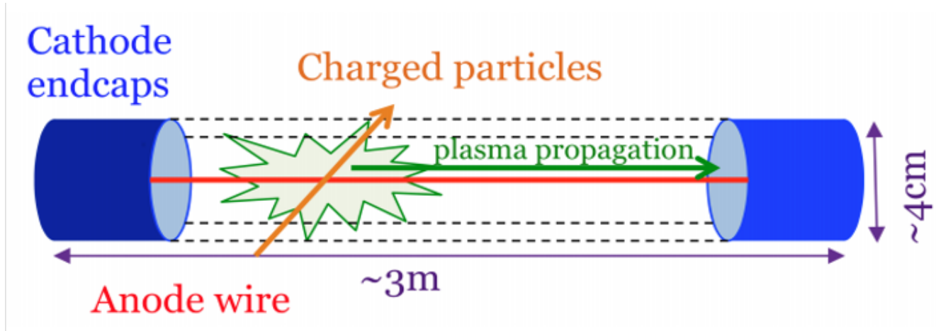
Figure 3.3: TrackerCells [43]
