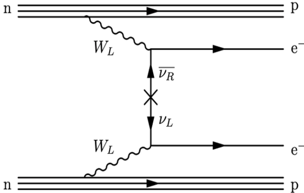
Figure 2.4: Feynman diagram for the forbidden neutrinoless double beta decay ( 0\nu\beta\beta ) via the light neutrino exchange (LNE) mechanism [16].
