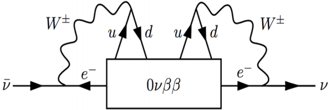
Figure 2.5: Feynman diagram for neutrinoless double beta decay ( 0\nu\beta\beta ), illustrating the Majorana nature of neutrinos for any intermediary decay mechanism [23].
