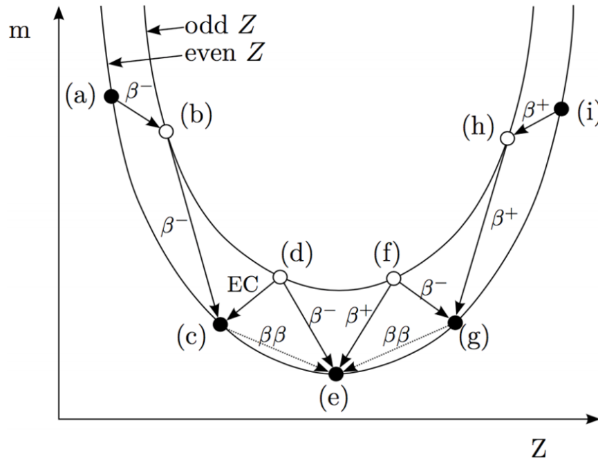
Figure 2.1: SEMF [16]
