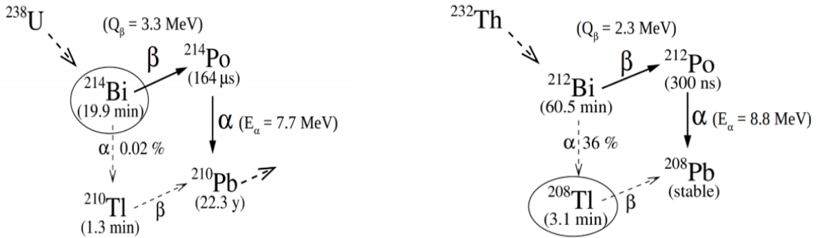
Figure 3.10: CloseDecayScheme [101]
