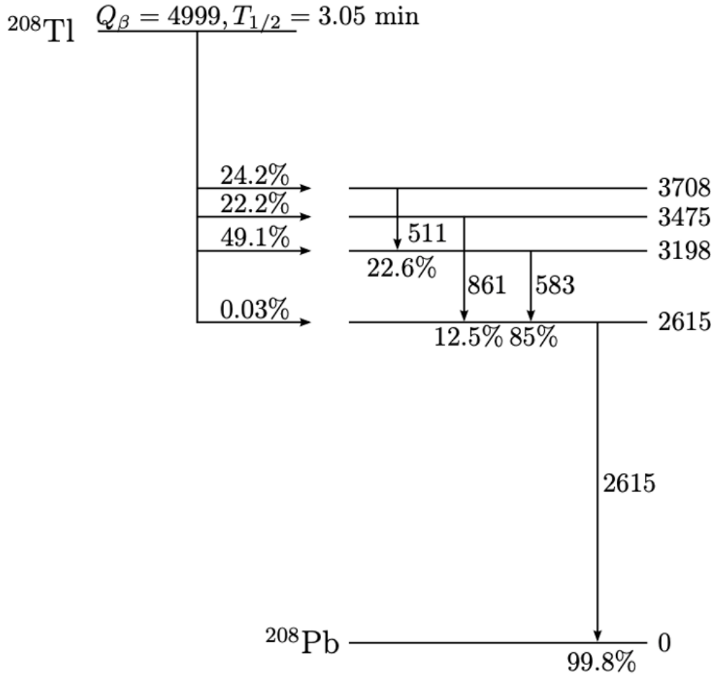
Figure 6.1: Simplified decay scheme for ^{208}\text{Tl} undergoing beta decay into ^{208}\text{Pb} , illustrating the most common transition lines, with the energies in keV [16].
