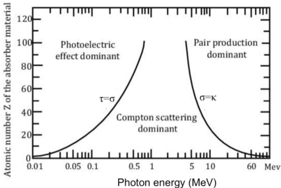
Figure 6.4: Cross section for photon interactions at various energies. The three principal interaction modes are shown as a function of the photon energy and atomic number of the interacting atom [42].
