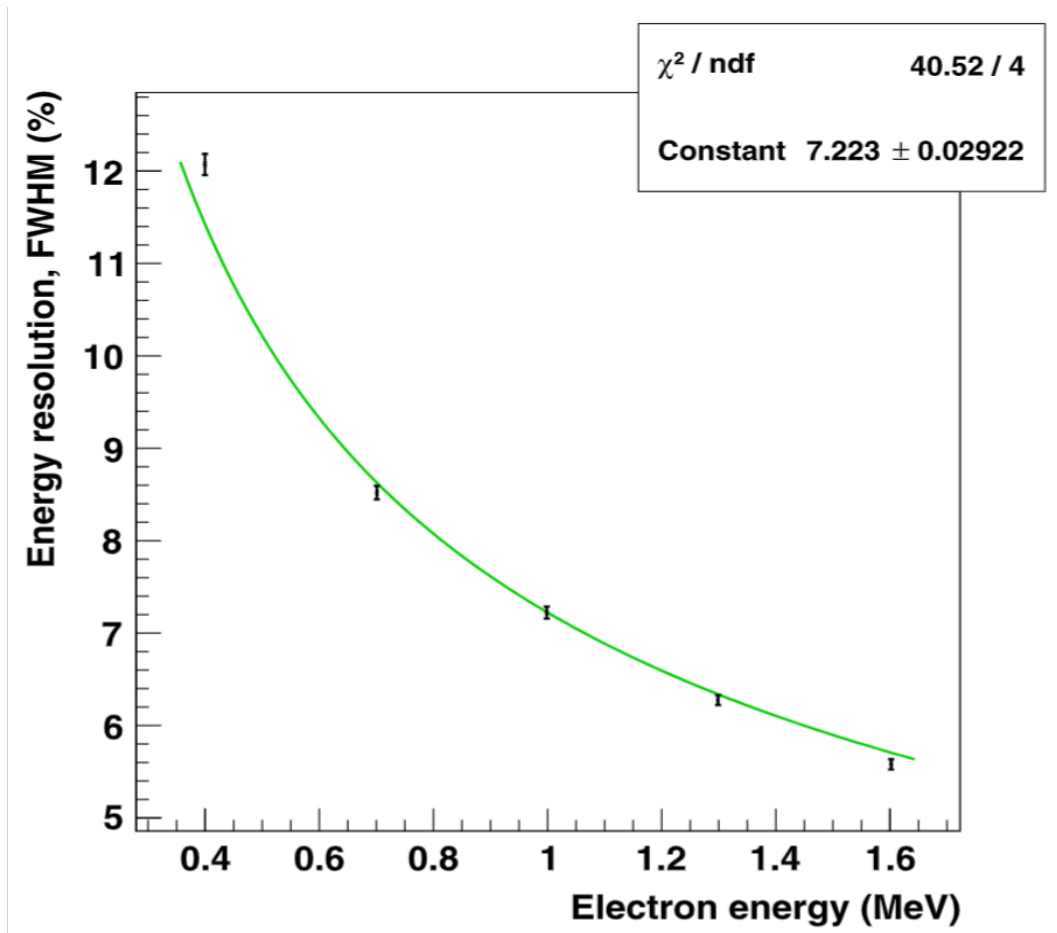
Figure 3.5: ResVsEnergy
