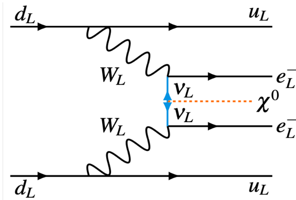
Figure 2.6: Feynman diagram for the forbidden neutrinoless double beta decay ( 0\nu\beta\beta ) via the emission of an associated Majoron ( \chi^0 ) [25].
