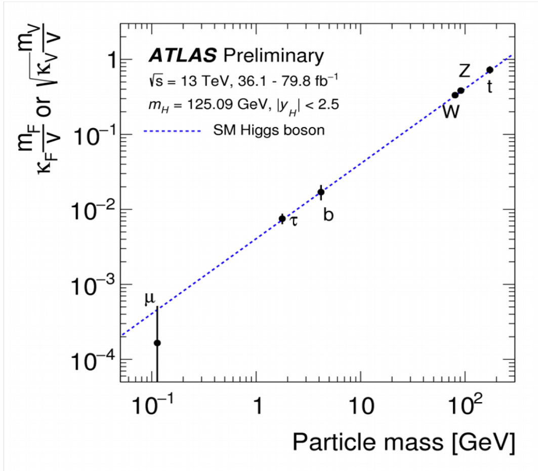
Figure 1.2: DiracCoupling [9]
