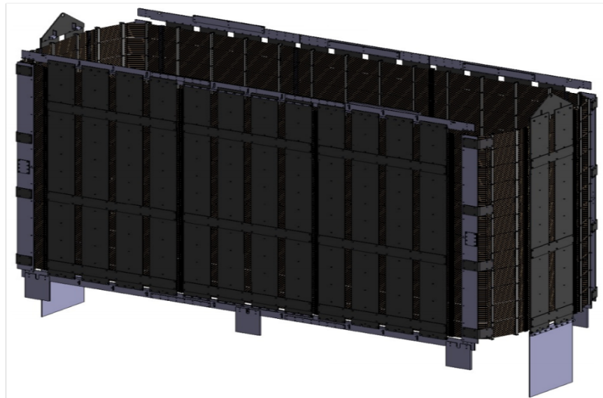
Figure 3.14: Overview of the assembled magnetic coil.
