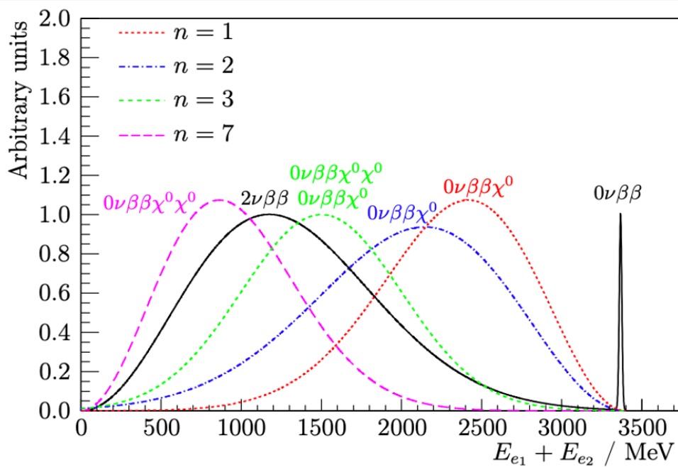
Figure 2.7: 0\nu\beta\beta and 2\nu\beta\beta energy spectra alongside four alternative Majoron decay modes with indices 1,2,3 and 7 [26].s
