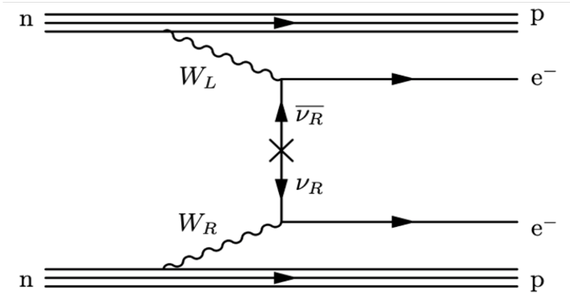
Figure 2.8: Feynman diagram for the forbidden neutrinoless double beta decay ( 0\nu\beta\beta ) via the \langle\lambda\rangle right handed weak current mechanism [33].
