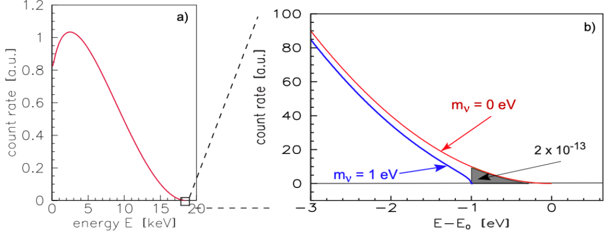
Figure 1.4: Tritium \beta decay energy spectrum illustrating the discrepancy in the high energy tail due to the emission of a massive 1 eV neutrino [16].
