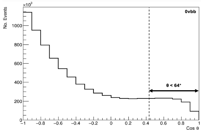
Figure 7.2: 0\nu\beta\beta angular distribution for events with a 2e topology and energy in the ^{82}\text{Se} ROI. The angular distribution is normalised to the number of simulated events and is only shown for the no field scenario. The calculated maximum angle for two charged particles striking adjacent calorimeters is shown by the dashed line.
