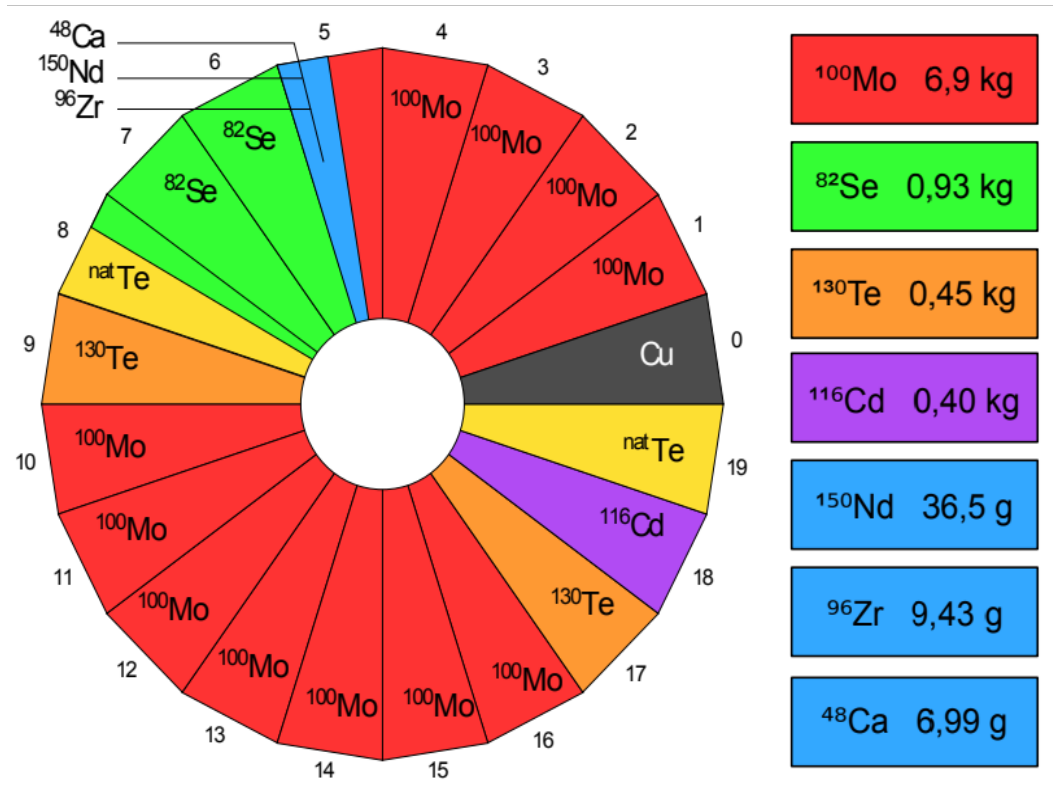
Figure 2.13: Distribution of source material across the 20 sections of the NEMO-3 detector [106].
