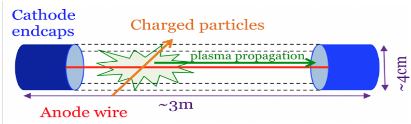
Figure 3.2: A SuperNEMO tracker cell illustrating detection principle [55].
