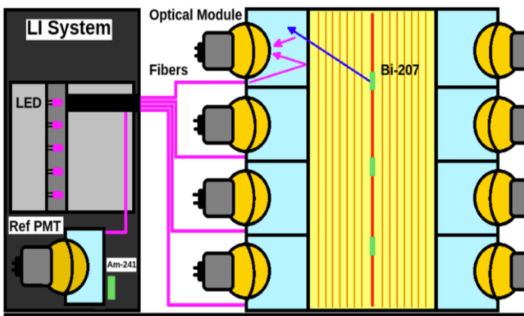
Figure 3.7: Illustration of the light injection monitoring system [120].
