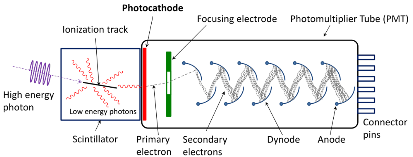
Figure 3.15: Schematic view of the working principle of a PMT coupled to a scintillator. The scintillation photons are focused within the PMT and read as an electric signal at the anode [123].
