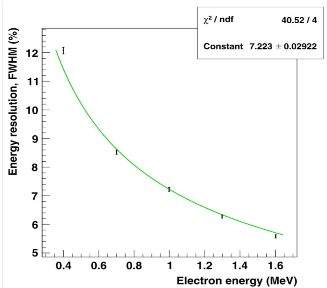
Figure 3.4: Energy resolution (FWHM %) as a function of the electron energy. Results were obtained using a ^{90}\text{Sr} based electron beam [59].
