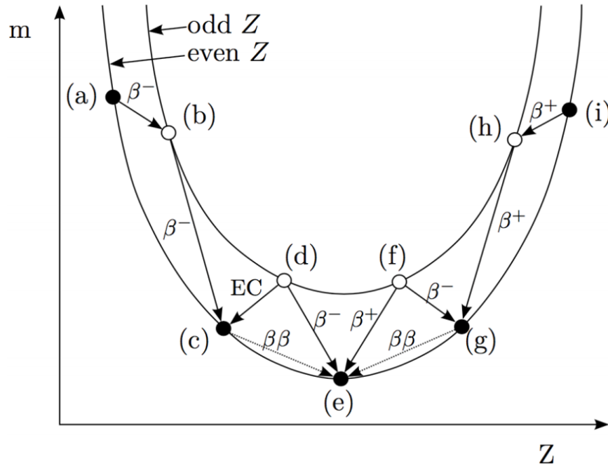
Figure 2.1: SEMF predictions for even values of A . The permitted decays are represented by arrows, with the decay mode labelled for each transition [7].
