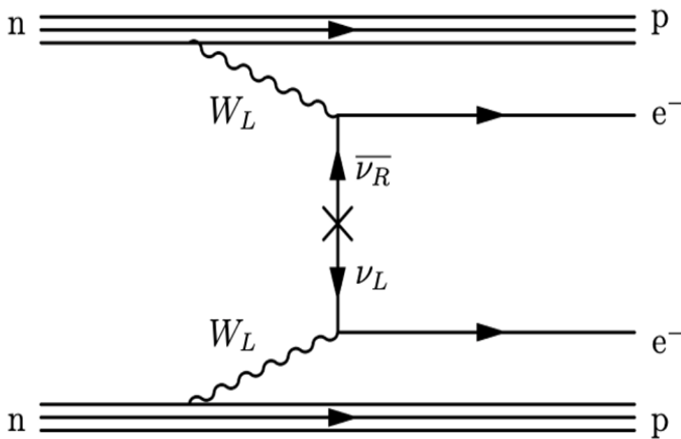
Figure 2.4: Feynman diagram for the forbidden neutrinoless double beta decay ( 0\nu\beta\beta ) via the light neutrino exchange (LNE) mechanism [7].
