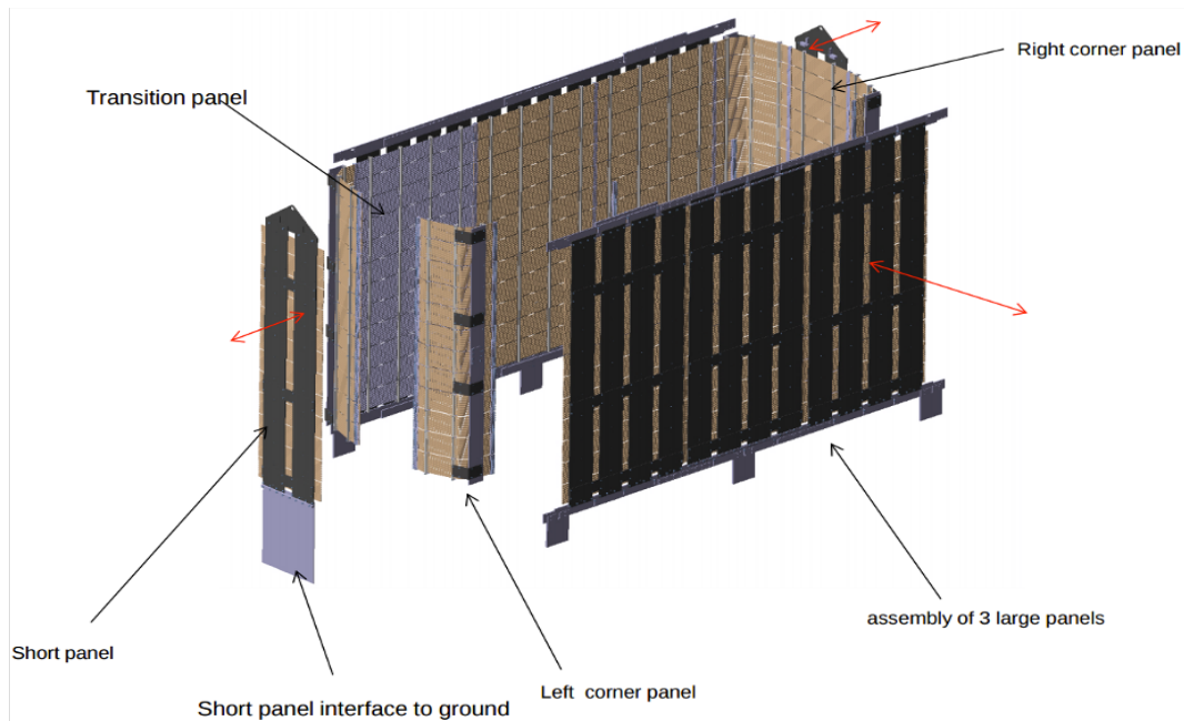
Figure 3.13: Open view of the magnetic coil illustrating the key components of the structure [121].
