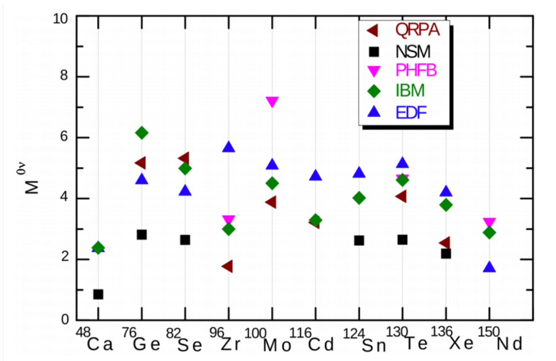
Figure 2.10: Nuclear matrix element (NME) values for the main double beta decaying isotopes used for experimentation, using the different methods described in Section 2.4 [44].
