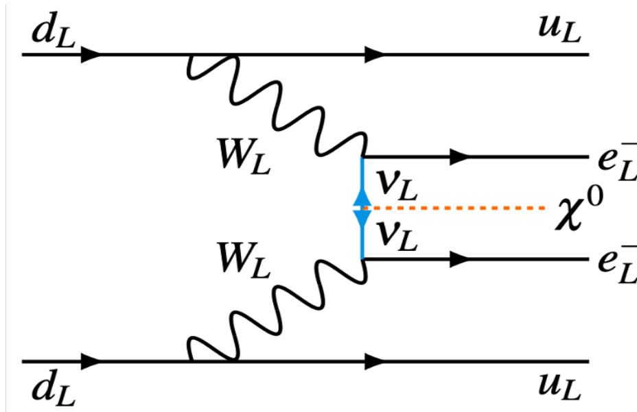
Figure 2.6: Feynman diagram for the forbidden neutrinoless double beta decay ( 0\nu\beta\beta ) via the emission of an associated Majoron ( \chi^0 ) [34].
