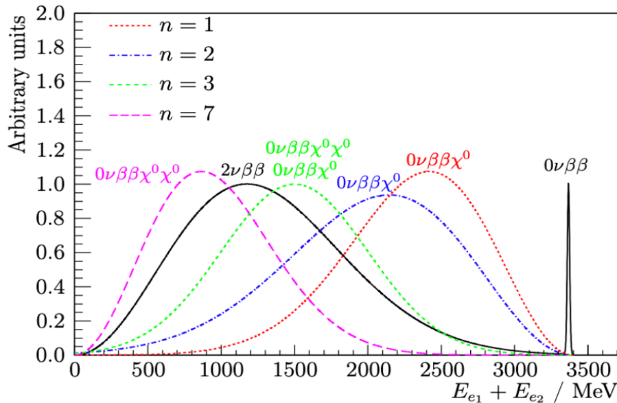
Figure 2.7: 0\nu\beta\beta and 2\nu\beta\beta energy spectra alongside four alternative Majoron decay modes with indices 1,2,3 and 7 [35]. s
