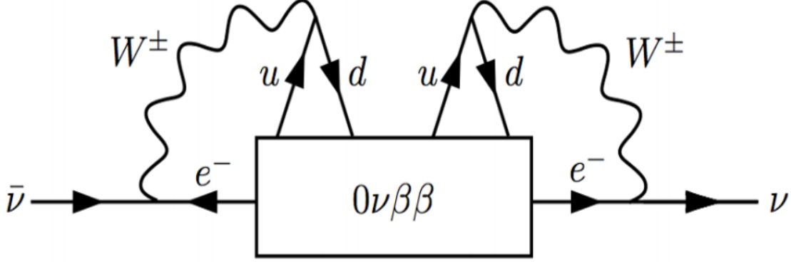
Figure 2.5: Feynman diagram for neutrinoless double beta decay ( 0\nu\beta\beta ), illustrating the Majorana nature of neutrinos for any intermediary decay mechanism [32].
