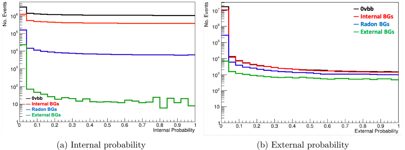
Figure 4.8: Internal (a) and external (b) probabilities for 0\nu\beta\beta , internal, radon and external backgrounds with reconstructed 2e topologies. The probability distributions were calculated using the equations 4.5 and 4.8 respectively.
