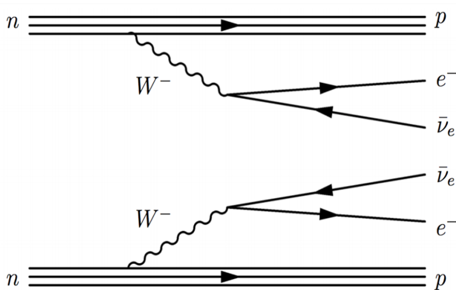
Figure 2.2: Feynman diagram for the Standard Model two neutrino double beta decay ( 2\nu\beta\beta ) [7].
