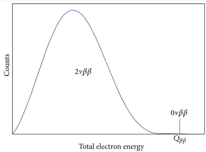
Figure 2.3: 0\nu\beta\beta and 2\nu\beta\beta theoretical electron energy spectra. 0\nu\beta\beta is represented by a single monochromatic line [31].
