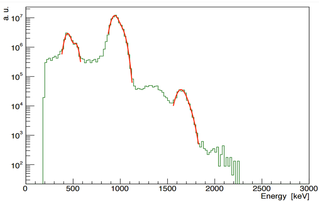
Figure 3.6: Reconstructed ^{207}\text{Bi} energy spectrum from a simulated calibration run. The three peaks correspond to the 482, 976 and 1682 keV energy lines [109].
