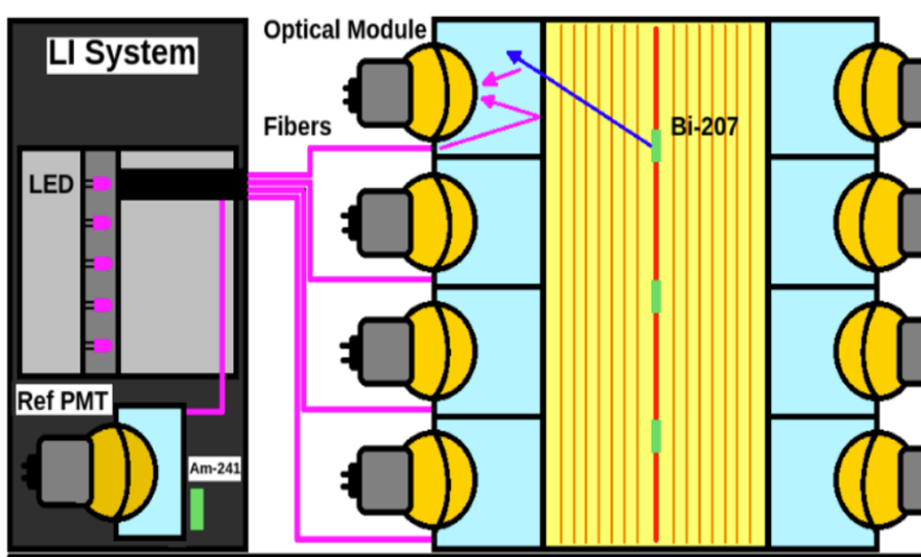
Figure 3.7: Illustration of the light injection monitoring system [110].
