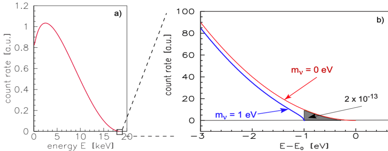
Figure 1.4: Tritium \beta decay energy spectrum illustrating the discrepancy in the high energy tail due to the emission of a massive 1 eV neutrino [13].
