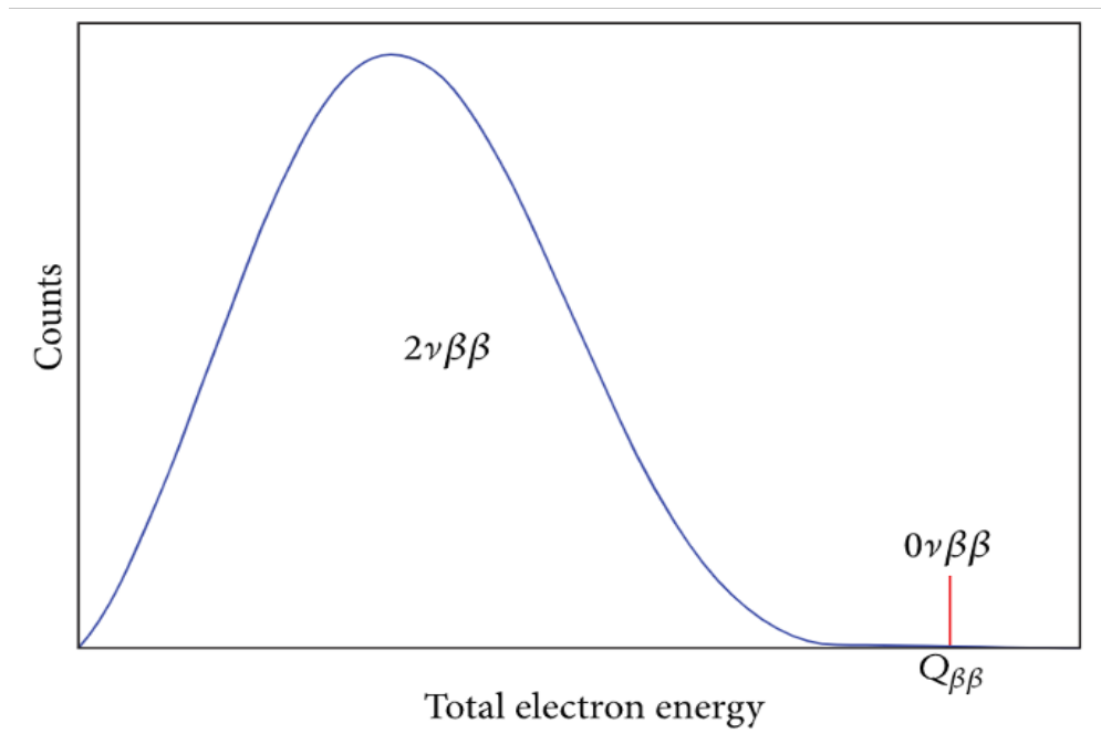
Figure 2.3: 0\nu\beta\beta and 2\nu\beta\beta theoretical electron energy spectra. 0\nu\beta\beta is represented by a single monochromatic line [25].
