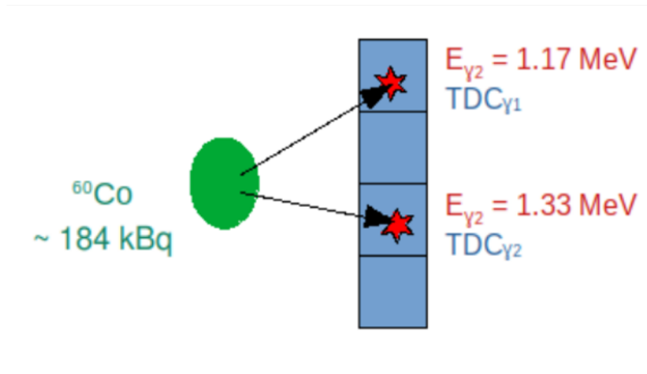
Figure 3.8: Schematic view of the time calibration system using ^{60}\text{Co} placed behind the calorimeter wall. The two gammas emitted from ^{60}\text{Co} are represented by the two arrows [41].
