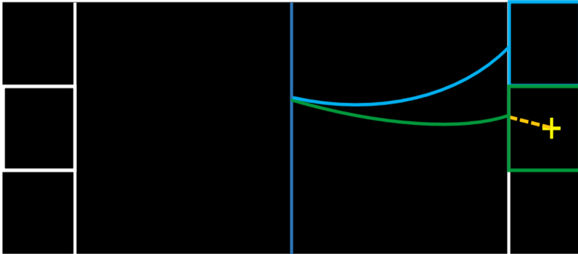
Figure 7.2: Representation of a reconstructed event with two charged particle tracks, the first belonging to an electron (blue track) and the second to a positron (green track), with an initial decay vertex on the source foil.
