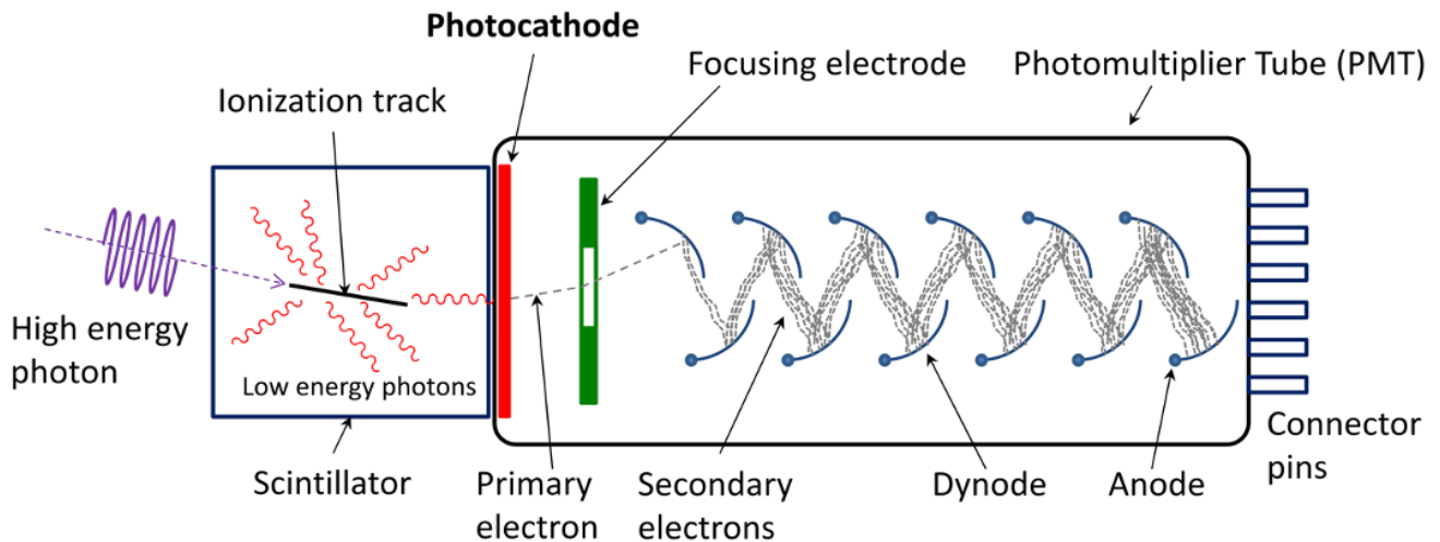
Figure 3.16: Schematic view of the working principle of a PMT coupled to a scintillator. The scintillation photons are focused within the PMT and read as an electric signal at the anode [113].
