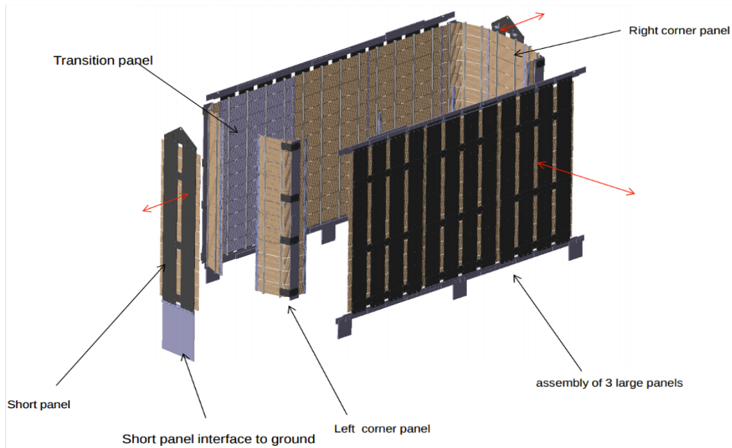
Figure 3.14: Open view of the magnetic coil illustrating the key components of the structure [111].
