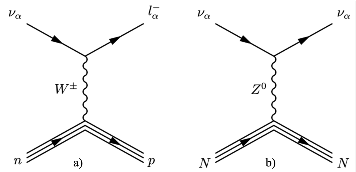
Figure 1.1: Feynman diagrams of neutrino interactions used to detect neutrinos. Interaction a) is a Charged Current (CC) neutrino-neutron scattering and interaction b) is a Neutral Current (NC) neutrino-neutron scattering [6].
