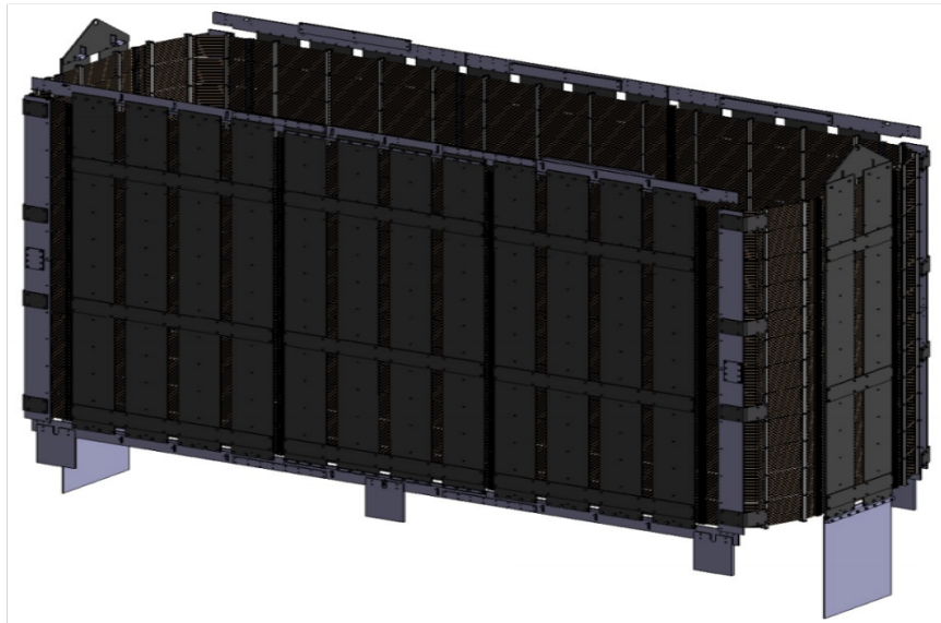
Figure 3.13: Overview of the assembled magnetic coil [111].
