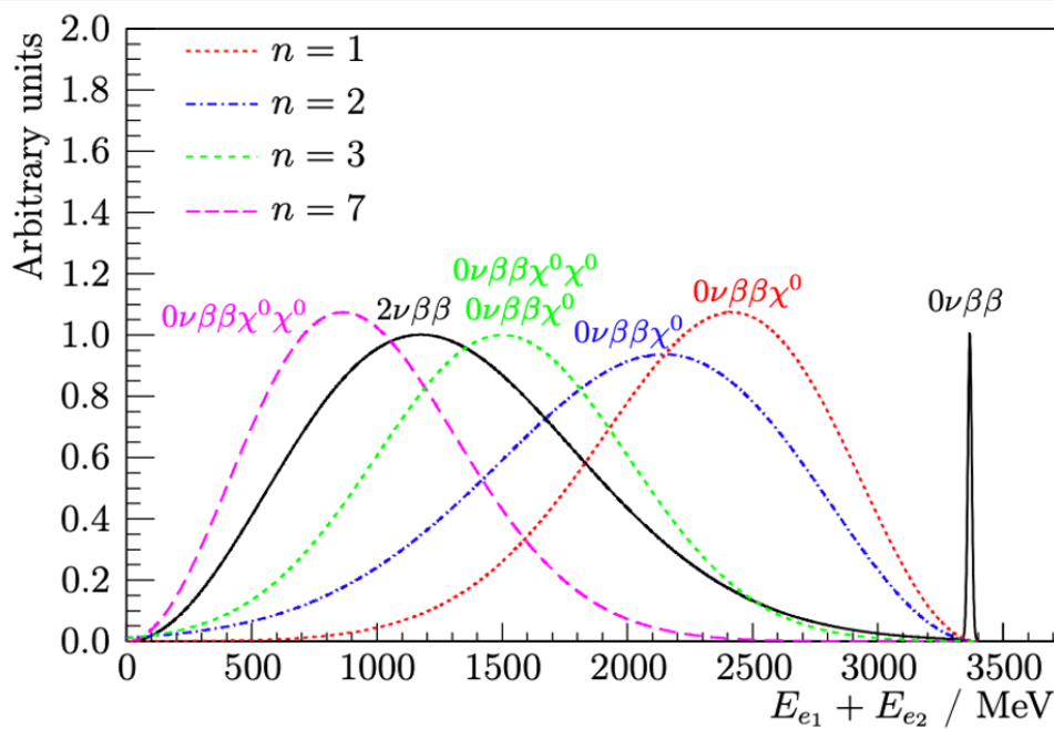
Figure 2.7: 0\nu\beta\beta and 2\nu\beta\beta energy spectra alongside four alternative Majoron decay modes with indices 1,2,3 and 7 [29].s
