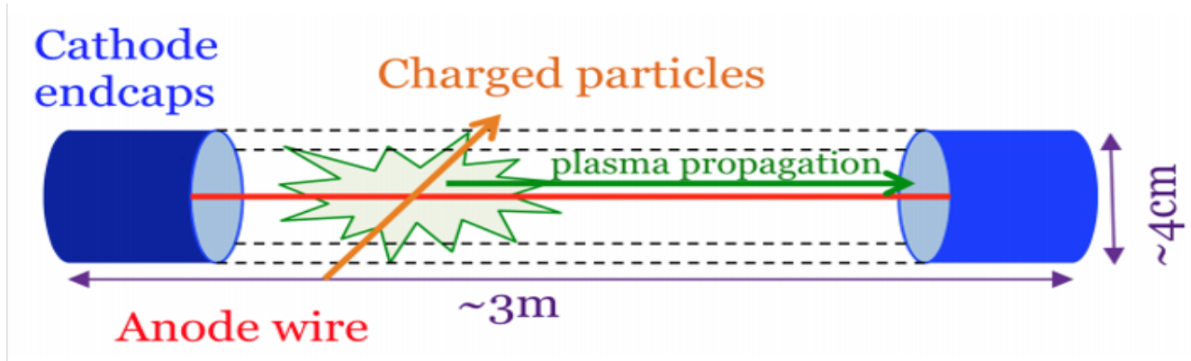
Figure 3.2: A SuperNEMO tracker cell illustrating detection principle [46].
