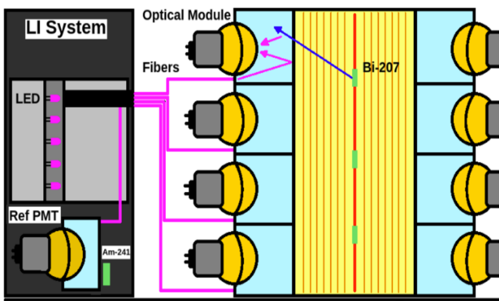
Figure 3.7: Illustration of the light injection monitoring system [116].
