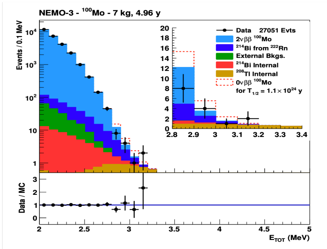
Figure 2.14: Energy distribution of ^{100}\text{Mo} double beta candidate events as well as the background contributions in the ^{100}\text{Mo} ROI [103]. The exposure for ^{100}\text{Mo} is 34.4 kg yrs.
