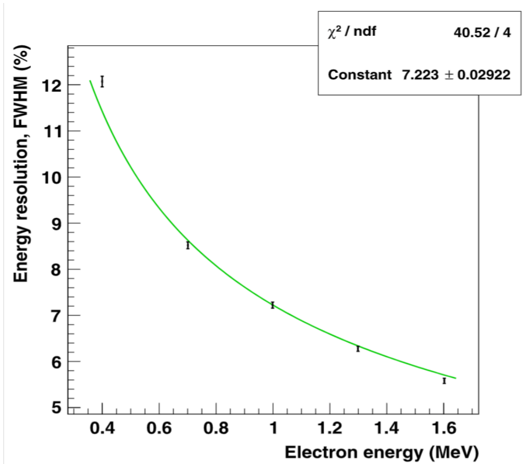
Figure 3.4: Energy resolution (FWHM %) as a function of the electron energy. Results were obtained using a ^{90}\text{Sr} based electron beam [55].
