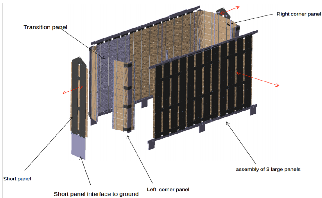
Figure 3.13: Open view of the magnetic coil illustrating the key components of the structure [117].
