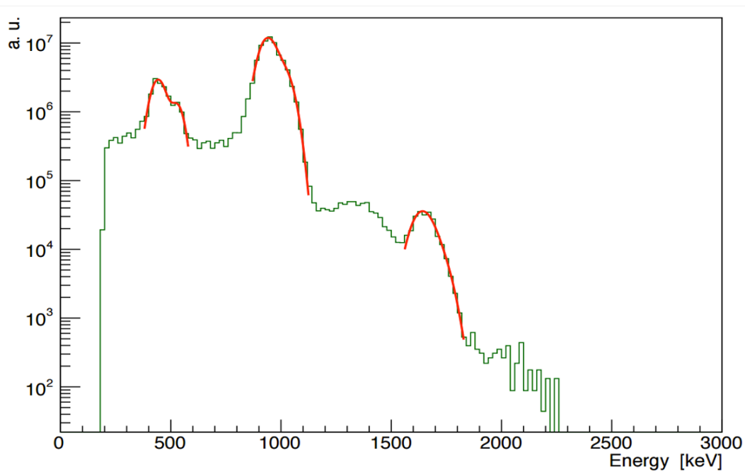
Figure 3.7: 207 Bi Spectrum
