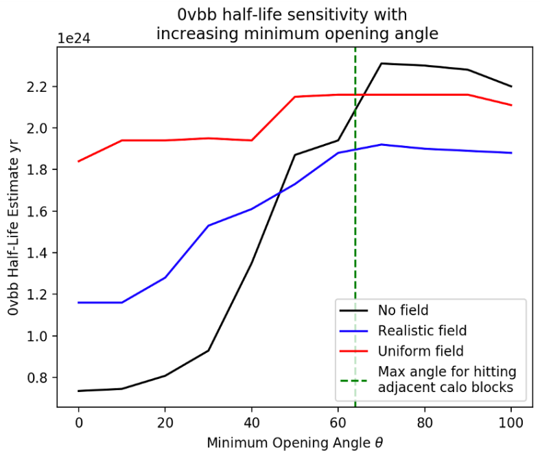
Figure 7.4: Minimum opening angle vs sensitivity for the three magnetic field configurations. Maximal sensitivity is achieved around a minimum angle of 70^\circ .
