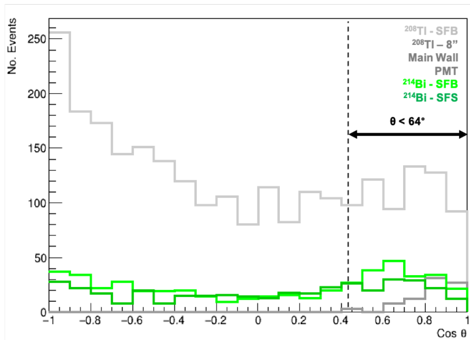
Figure 7.3: \text{Cos } \theta distribution for different backgrounds, including the theoretical maximum angle for two charged particles striking adjacent calorimeters (dashed line).
