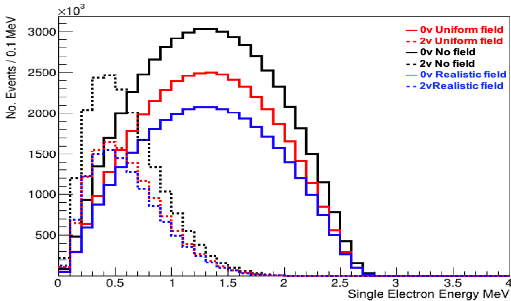
Figure 5.2: 0\nu and 2\nu\beta\beta single electron energy spectra for events with a 2e topology with all three magnetic fields. The 0\nu\beta\beta spectra are illustrated by the thick line and 2\nu\beta\beta by the dotted line.
