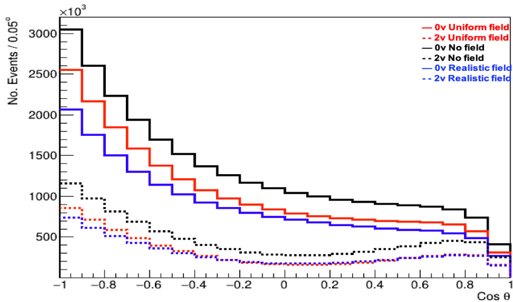
Figure 5.3: 0\nu and 2\nu\beta\beta \cos\theta spectra for events with a 2e topology with all three magnetic fields. The 0\nu\beta\beta spectra are illustrated by the thick line and 2\nu\beta\beta by the dotted line. All events have a total energy within the ^{82}\text{Se} ROI (2.8 - 3.2 MeV).
