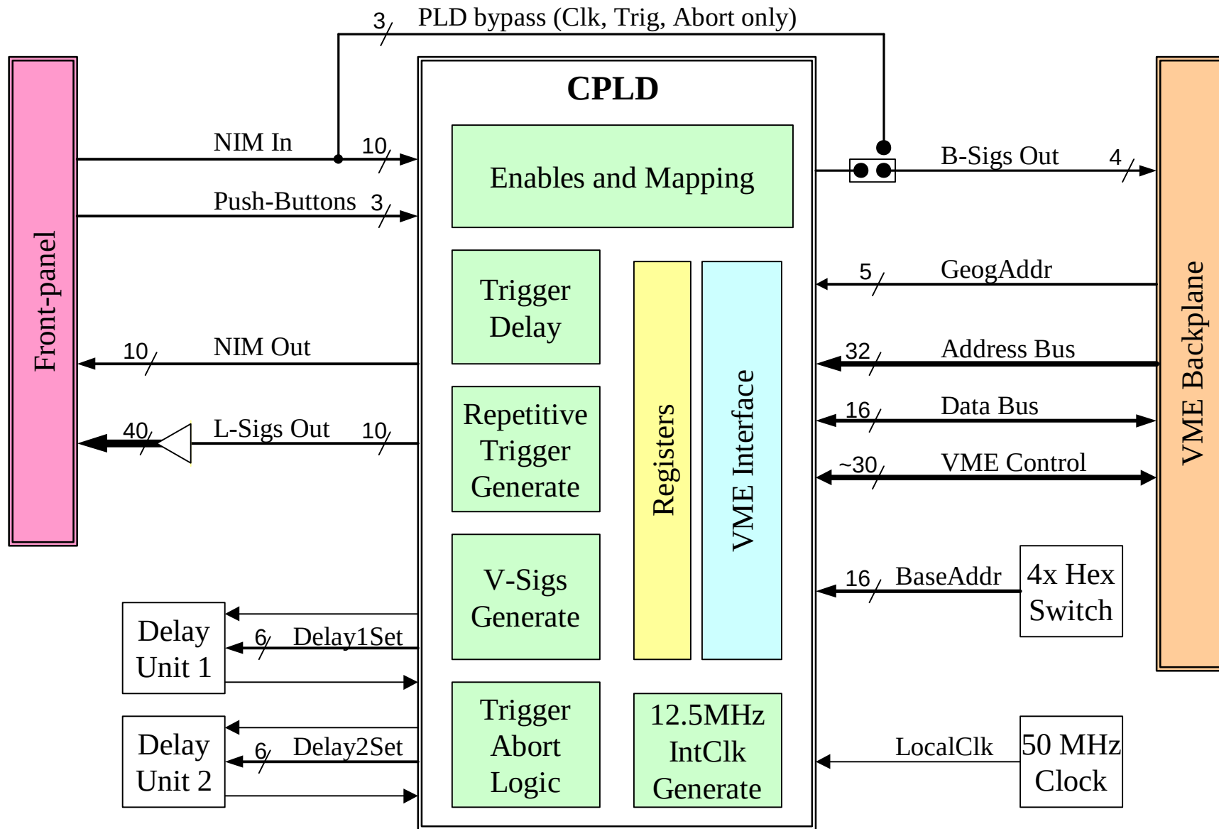
Trigger Board Block Diagram
