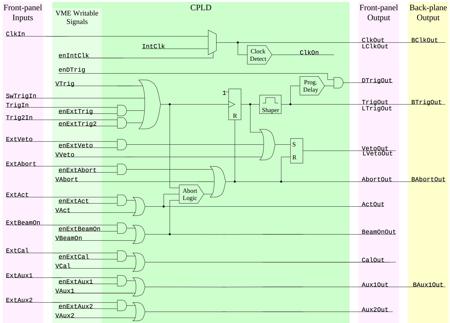
Trigger Board Functional Diagram
